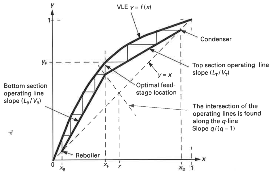
Figure 6 McCabe-Thiele diagram with an optimally located feed.
