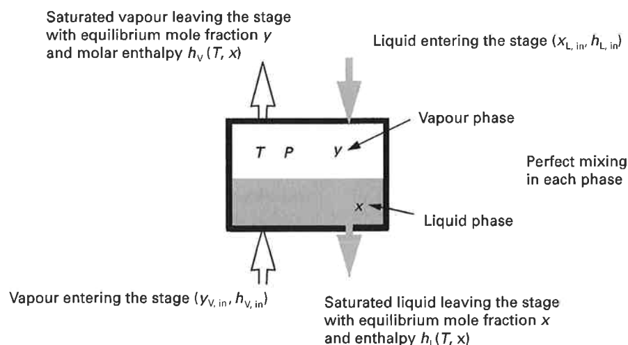
Figure 1 Equilibrium-stage concept.
