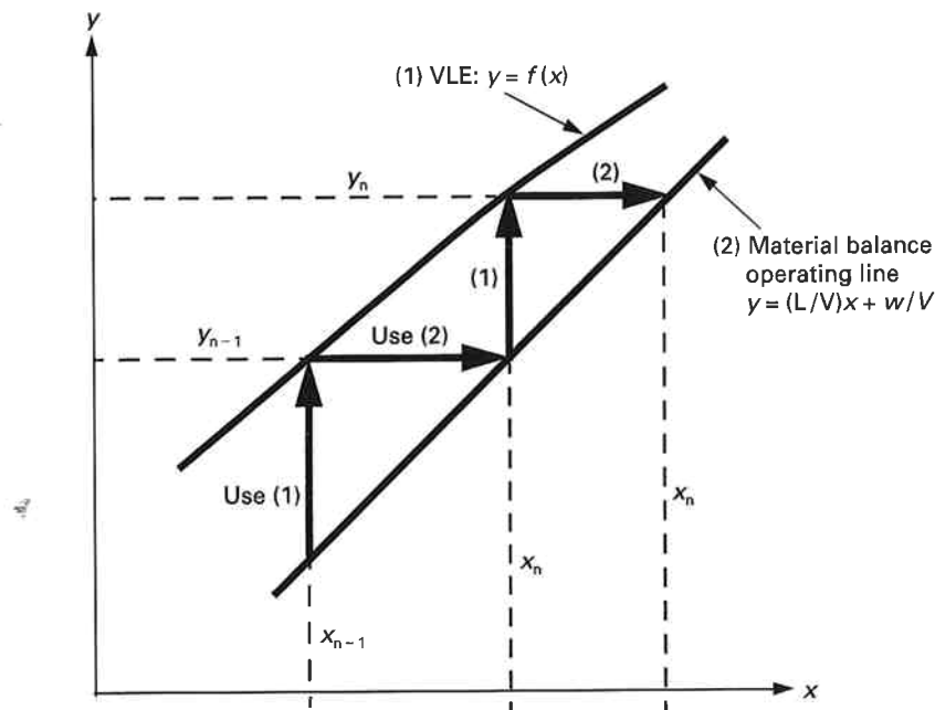
Figure 4 Combining the VLE and the operating line to compute mole fractions in a section of equilibrium stages.
