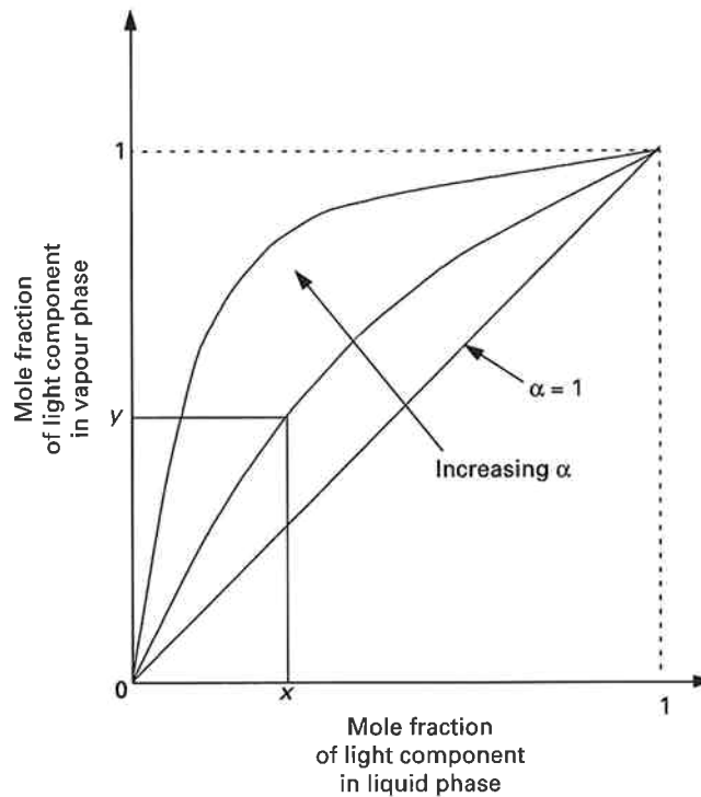
Figure 2 VLE for ideal binary mixture: y = \alpha x/1 + (\alpha - 1)x .
