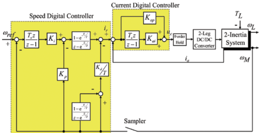
Figure 7. Proposed control system (discrete controller model).
