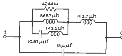
Fig. 25—Second interstage for the amplifier of Fig. 23.
