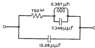
Fig. 27—Cathode impedance for the amplifier of Fig. 23.
