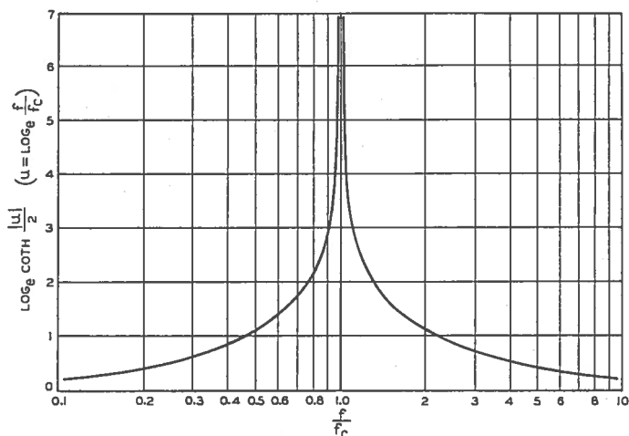
Fig. 2—Weighting function in loss-phase formula.
