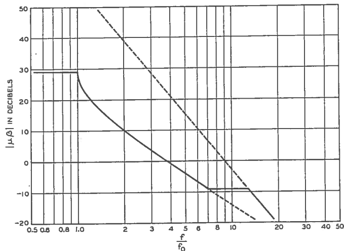
Fig. 16—Modified cutoff permitting 30° phase margin and 9 db gain margin.
