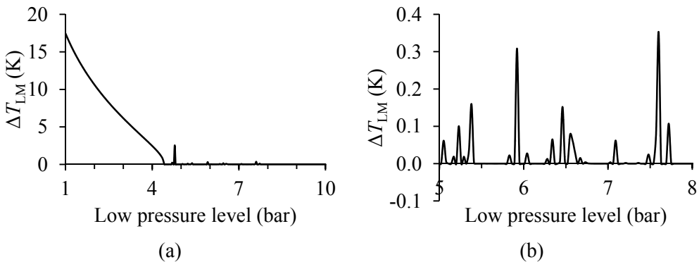
Figure 3.22. Logarithmic mean temperature difference in heat exchanger as function of low pressure level. (a) For the complete range; (b) for a range where the smallest temperature difference is less than zero.
