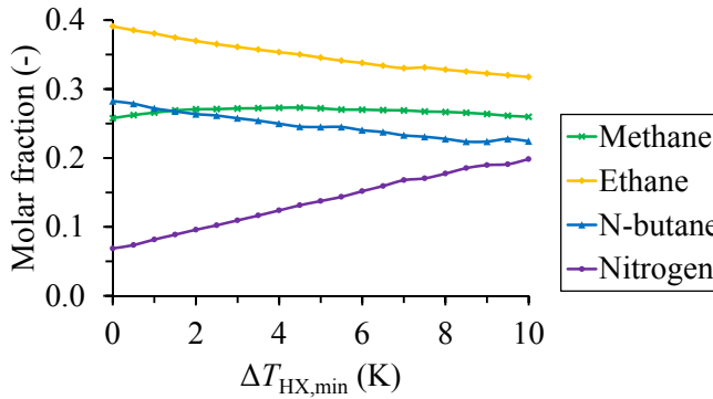
Figure 3.38. Molar composition of mixed refrigerant in best known solution as function of minimum temperature difference.
