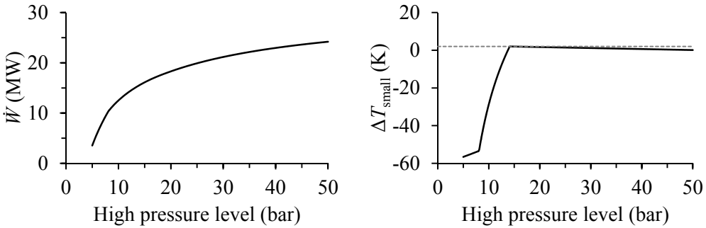
Figure 3.25. (a) Power consumption as function of high pressure level; (b) Smallest temperature difference in heat exchanger as function of high pressure level.
