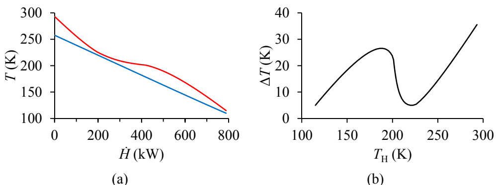
Figure 5.8. Composite curves for best known solution of rigorous model for single nitrogen expander process with \eta_s = 1.00 and \Delta T_{\min} = 5 K; (b) Temperature difference as function of hot stream temperature.
