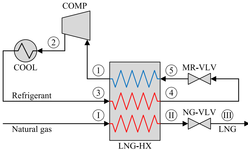
Figure 4.1. Process flowsheet for single mixed-refrigerant process.
