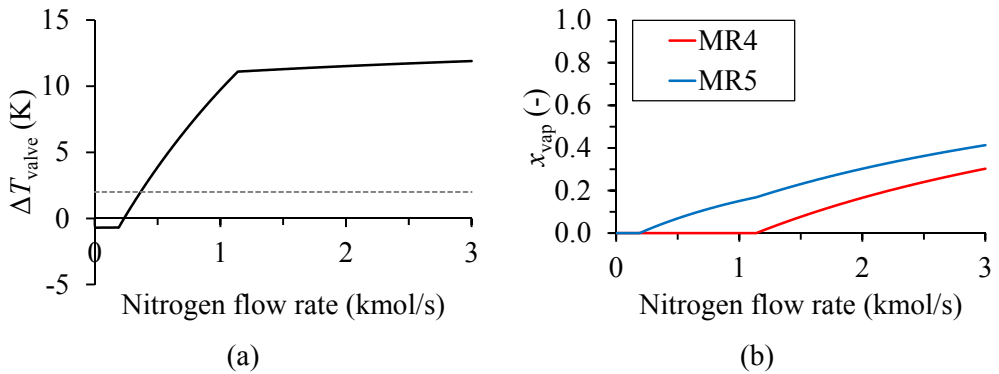
Figure 3.19. (a) Temperature difference across throttle valve as function of nitrogen flow rate; (b) Vapour fraction of refrigerant streams as functions of nitrogen flow rate.
