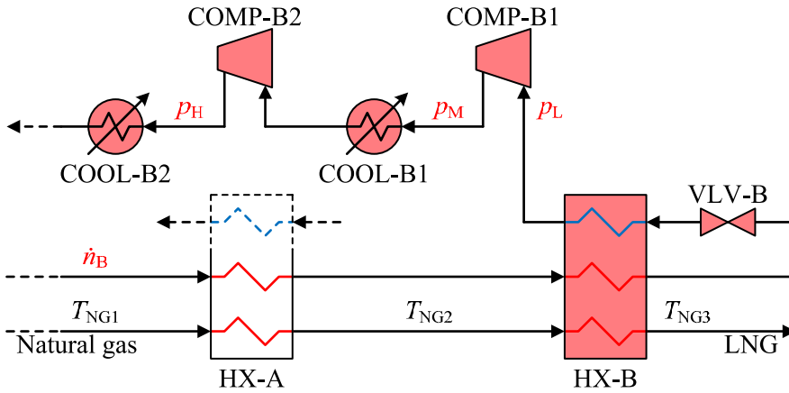
Figure 8.14. Mixed-refrigerant sub-cooling cycle with two-stage compression.
