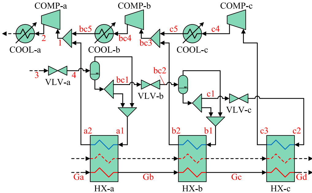
Figure 6.13. Flowsheet of vertical stage with three horizontal stages in pure-refrigerant cascade process.
