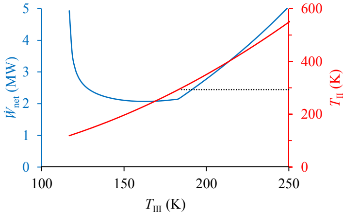
Figure 5.18. Net power consumption in simplified model of dual expander process as function of the stage temperature.
