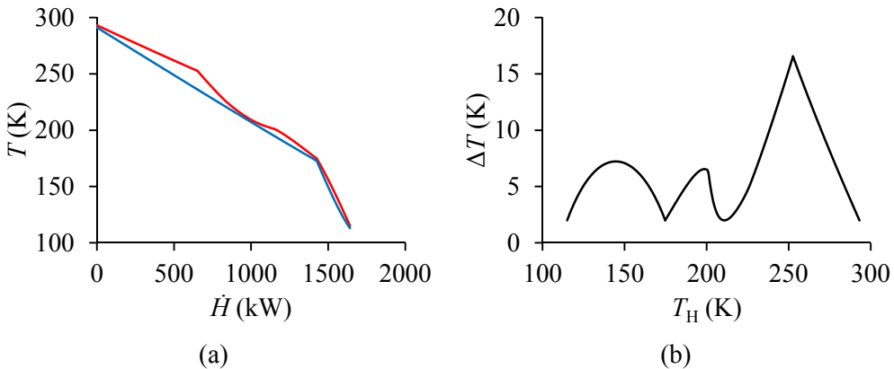
Figure 5.19. Composite curves for best known solution of rigorous model for dual nitrogen expander process with \eta_s = 0.80 and \Delta T_{\min} = 2 K; (b) Temperature difference as function of hot stream temperature.
