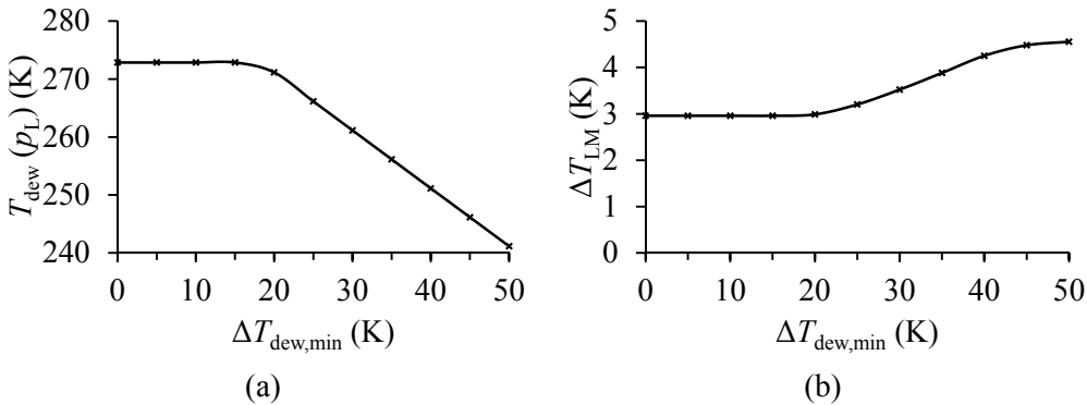
Figure 3.35. (a) Dew point temperature of compressor suction stream in best known solution as function of minimum temperature difference; (b) Logarithmic mean temperature difference in the heat exchanger for the best known solution as function of minimum superheating.
