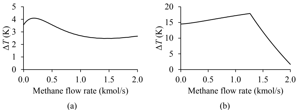
Figure 3.32. Temperature difference at two different points in the heat exchanger as function of the methane flow rate linearized with respect to temperature and extra evaluation points for phase change.
