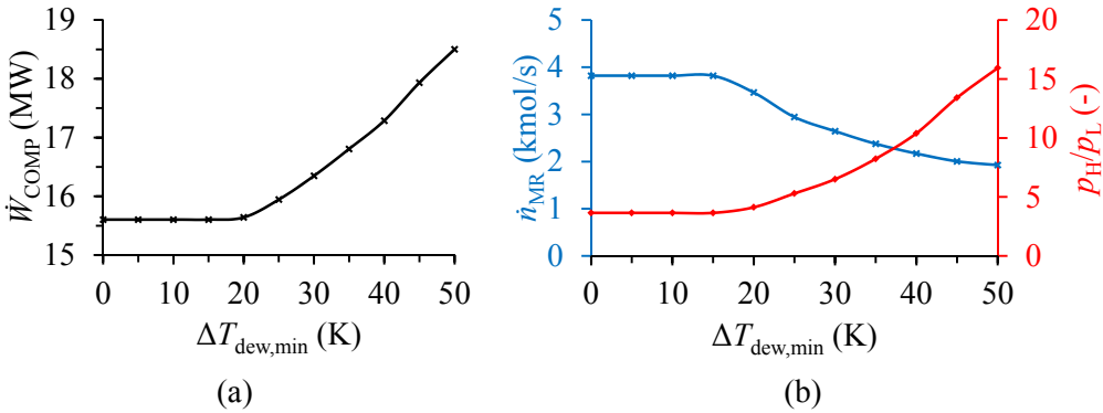
Figure 3.34. (a) Power consumption of best known solution as function of minimum superheating; (b) Refrigerant flow rate (blue) and pressure ratio (red) in best known solution as functions of minimum superheating.
