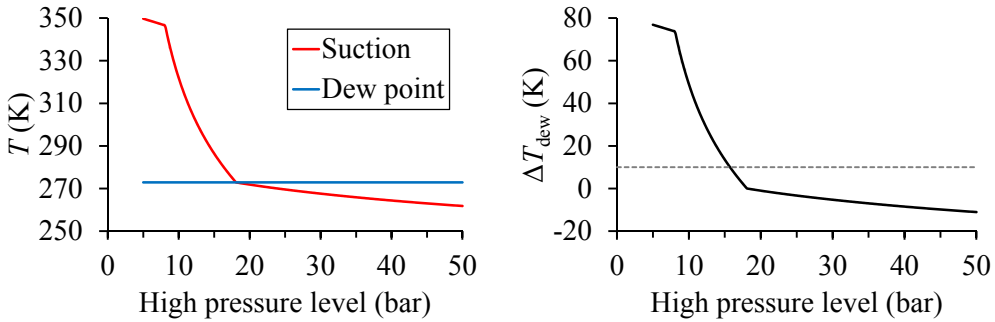
Figure 3.24. (a) Compressor suction temperature and refrigerant low pressure dew point as functions of high pressure level; (b) Compressor suction superheating as function of high pressure level.
