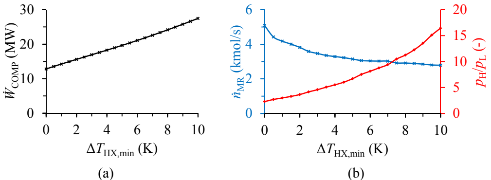
Figure 3.37. (a) Power consumption of best known solution as function of minimum temperature difference; (b) Refrigerant flow rate (blue) and pressure ratio (red) in best known solution as functions of minimum temperature difference.
