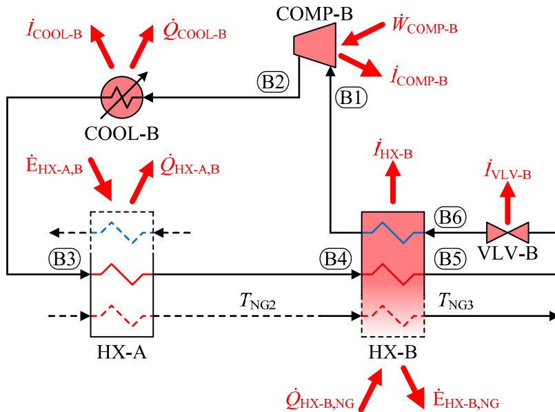
Figure 8.4. Energy and exergy balance for the sub-cooling cycles in a mixed-refrigerant process with two vertical stages and one horizontal stage each.
