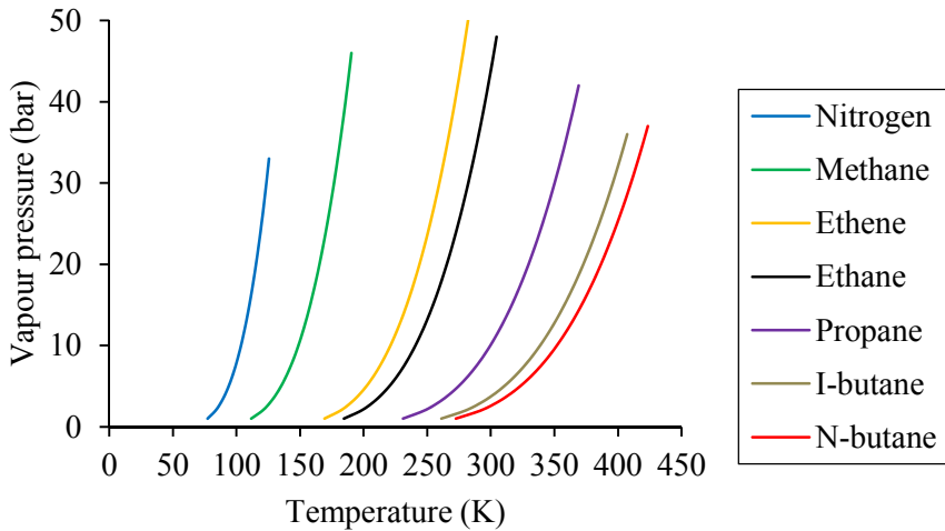
Figure 6.2. Saturation pressure as function of temperature for different refrigerant alternatives.
