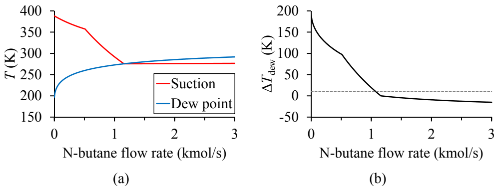
Figure 3.11. (a) Compressor suction temperature and refrigerant low pressure dew point as functions of n-butane flow rate; (b) Compressor suction superheating as function of n-butane flow rate.
