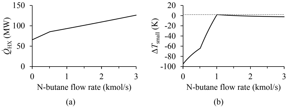
Figure 3.14. (a) Heat exchanger cooling load as functions of n-butane flow rate; (b) Smallest temperature difference in heat exchanger as function of n-butane flow rate.
