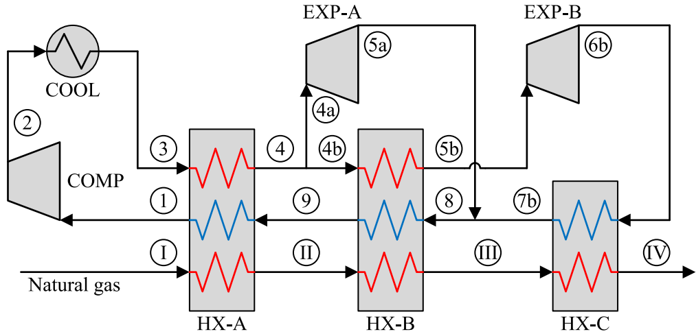
Figure 5.16. Dual expander process flowsheet.
