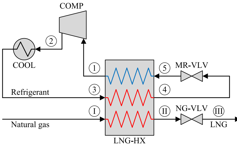
Figure 3.1. Flowsheet for single mixed-refrigerant LNG process.
