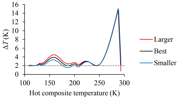
Figure 3.6. Temperature difference in the heat exchanger of a simple PRICO ® process for different values of the methane flow rate. Minimum temperature difference indicated by the dotted line.
