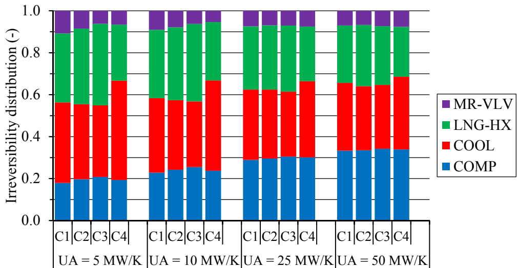
Figure 7.14. Irreversibility distribution between unit operations in best solution obtained from the different constraint formulations for different UA values.
