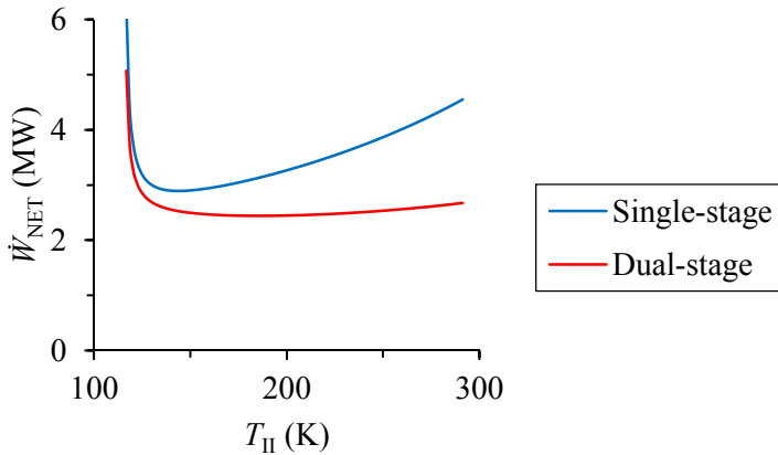
Figure 5.15. New power consumption in single expander process for natural gas liquefaction with one (blue) and two (red) stages of compression.
