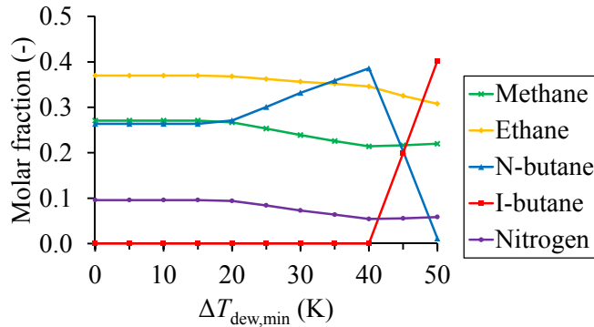
Figure 3.36. Molar composition of mixed refrigerant in best known solution as function of minimum superheating.
