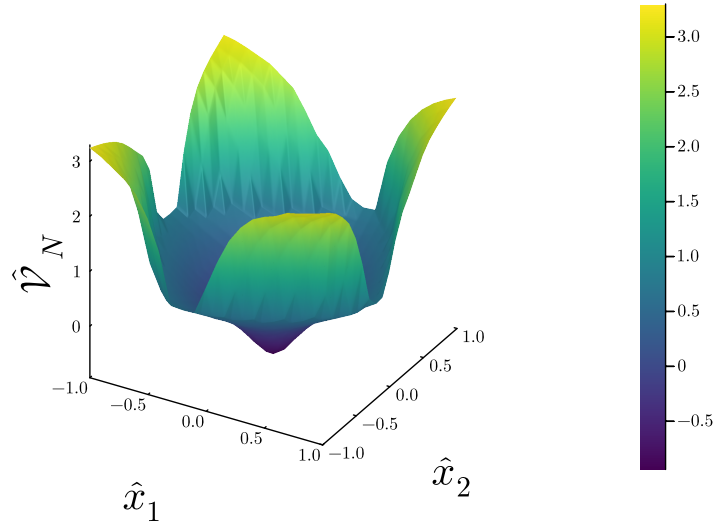
Figure 6.4: Cost-to-go using the ICNN with 1 horizon.
