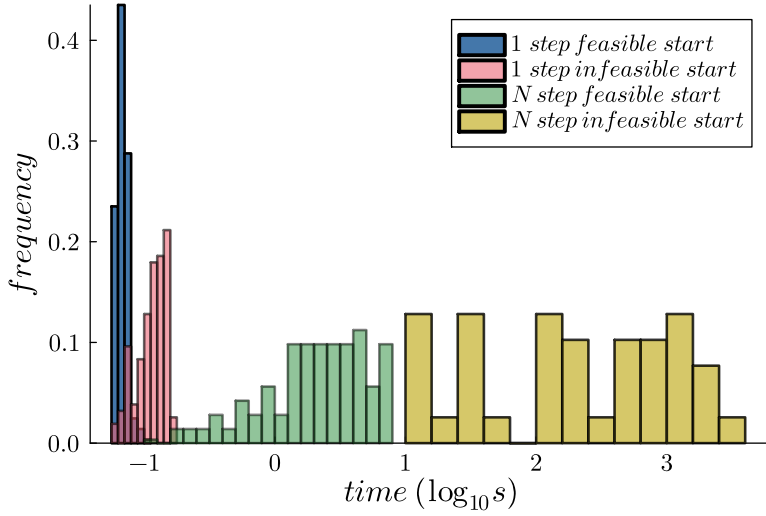
Figure 6.2: Solve times with the interpolating convex functions.
