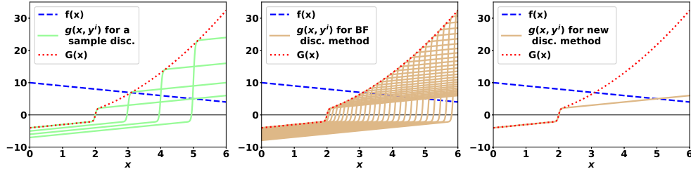
Figure 9.1: Benefits of bounding-focused discretization: Left: objective f(x) and constraint G(x) for Example 4 along with discretization Y_d = \{2, 3, 4, 5\} (cf. [13, Figure 3.1]). Middle: BF method needs 27 discretization points for its lower bounds to converge to v^* . Right: our proposed bounding-focused discretization method in Section 9.3 only requires a single discretization point ( |Y_d| = 1 ).
