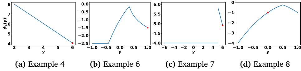
Figure 9.2: Value functions \phi_1 (note the discontinuity for Example 7). The red dot indicates \phi_1 at the point y^{BF,1} determined by the BF algorithm at iteration 1.
