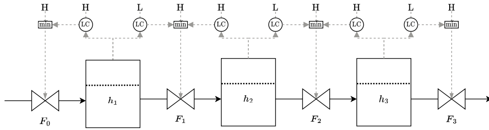
Figure 4.1: Three tanks in series, with bidirectional inventory control structure proposed by Zotică et al. [2] in grey. The grey dashed lines represent control signals, LC represent a level controller, and the min blocks represent min selectors. H and L represent high and low limits, of their corresponding LC or min selector. We neglect a subscript to show their relationship as this is clear from context. The level setpoints vary between the high and low limits automatically to isolate the effects of the current, and future, bottlenecks.
