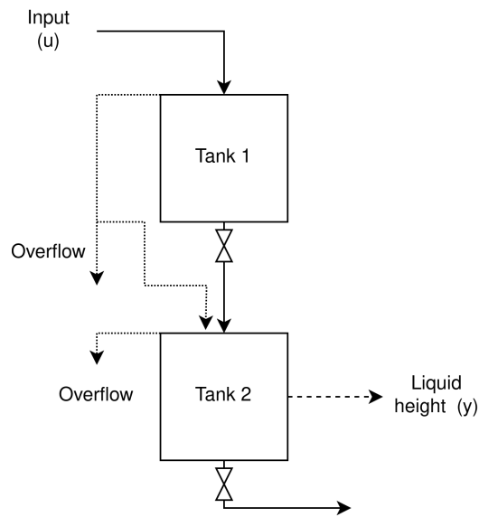
Figure 8.5: Diagram of cascading tank system
