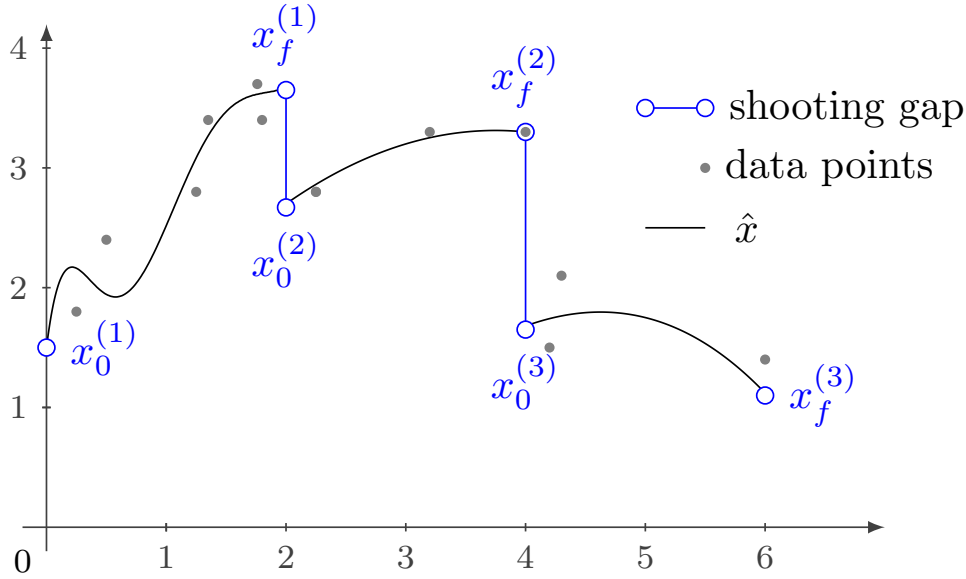
Figure 8.2: Schematic of multiple shooting.
