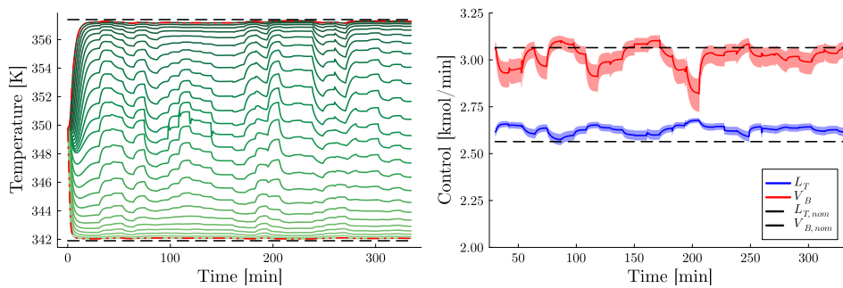
(a) Temperature profile (constant bias)
