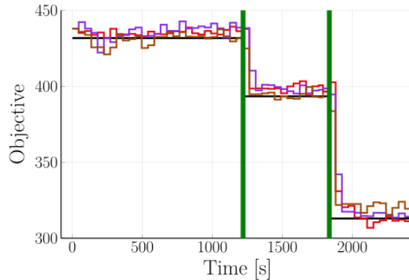
Figure C.1: Average objective value (45 seconds) of the methods compared the average profit achieved by using the quadratic model without modifications (black line). MA is in red, GP-MAY in purple, and GP-RTO in brown. Different operating sections (due to step-disturbances) are separated by vertical green lines.
