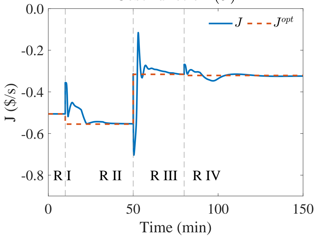
Cost function ( J )
