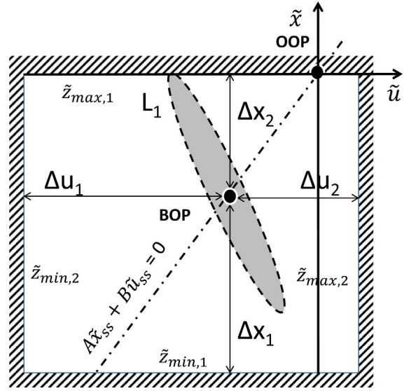
Fig. 2. Non-optimal controller design (solution from stage 1).
