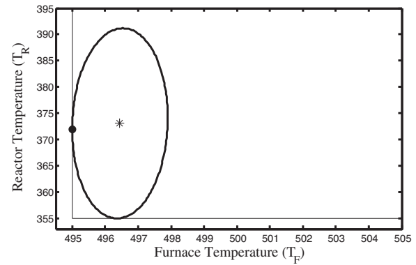
Fig. 7. Furnace temperature vs reactor temperature.
