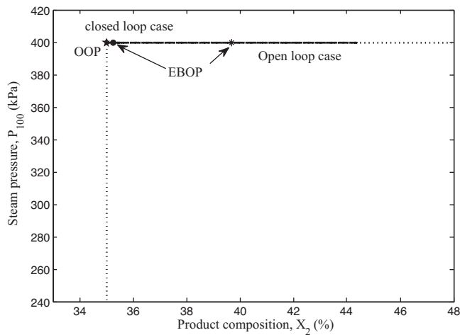
Fig. 16. Product composition vs steam pressure.
