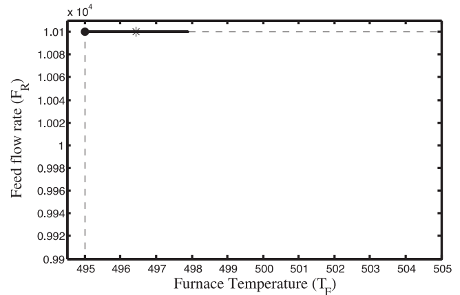
Fig. 8. Furnace temperature vs feed flow rate.
