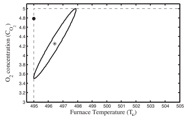
Fig. 10. Furnace temperature vs O 2 concentration.
