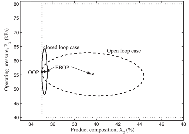
Fig. 14. Product composition vs operating pressure. (a) Open loop case: F_3 and F_{200} are constant. (b) Closed loop case: F_3 and F_{200} are used for control of X_2 .
