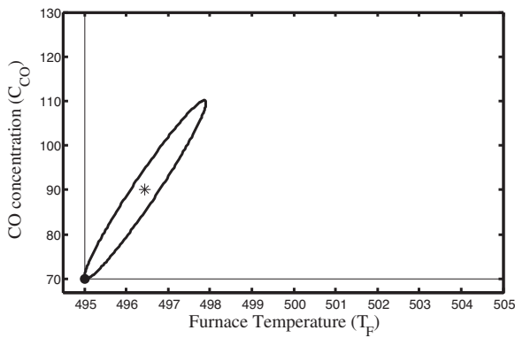
Fig. 11. Furnace temperature vs CO concentration.
