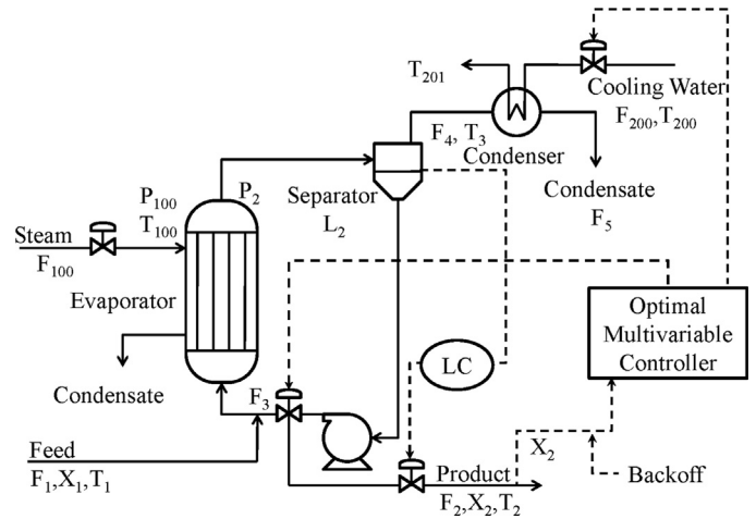
Fig. 13. Evaporator system.
