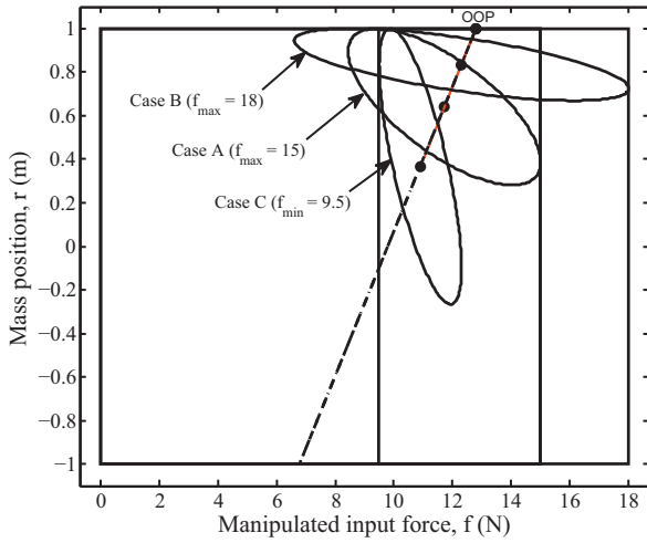
Fig. 5. Impact of change in constraint for mass spring damper system.
