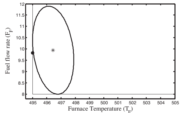
Fig. 9. Furnace temperature vs fuel flow rate.
