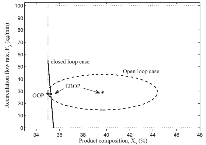
Fig. 15. Product composition vs recirculation flow rate.
