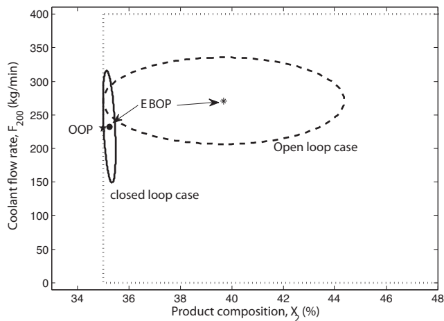
Fig. 17. Product composition vs coolant flow rate.
