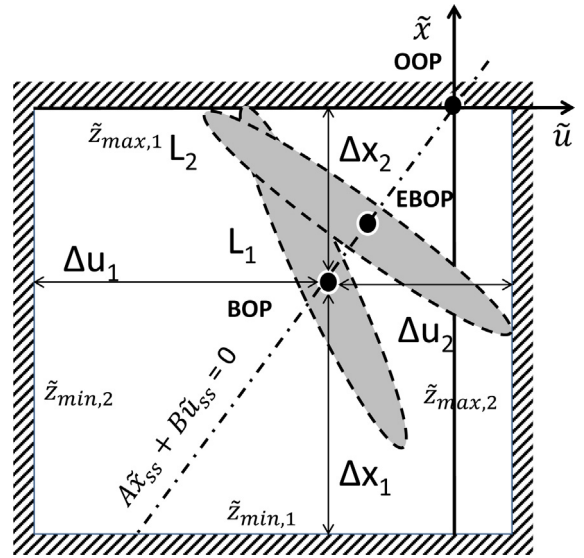
Fig. 3. Optimal controller design (after convergence).
