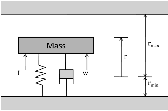
Fig. 4. Mass spring damper system.
