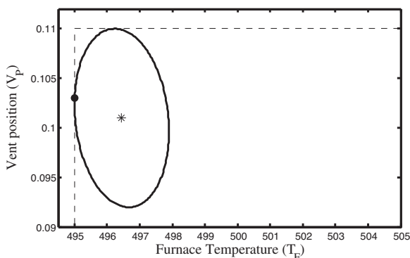
Fig. 12. Furnace temperature vs vent position.
