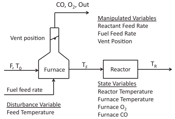
Fig. 6. Preheating furnace reactor system.
