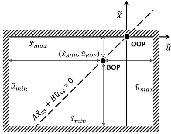
Fig. 1. Feasible region: dynamic (box) and steady state (dashed line).
