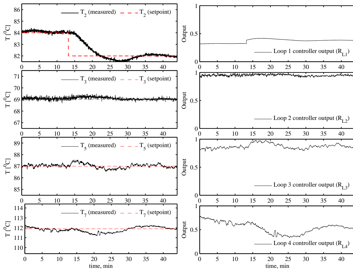
Figure 6: Experimental Run 2: -2[^\circ\text{C}] setpoint change in prefractionator temperature, T 2 (control loop 1)
