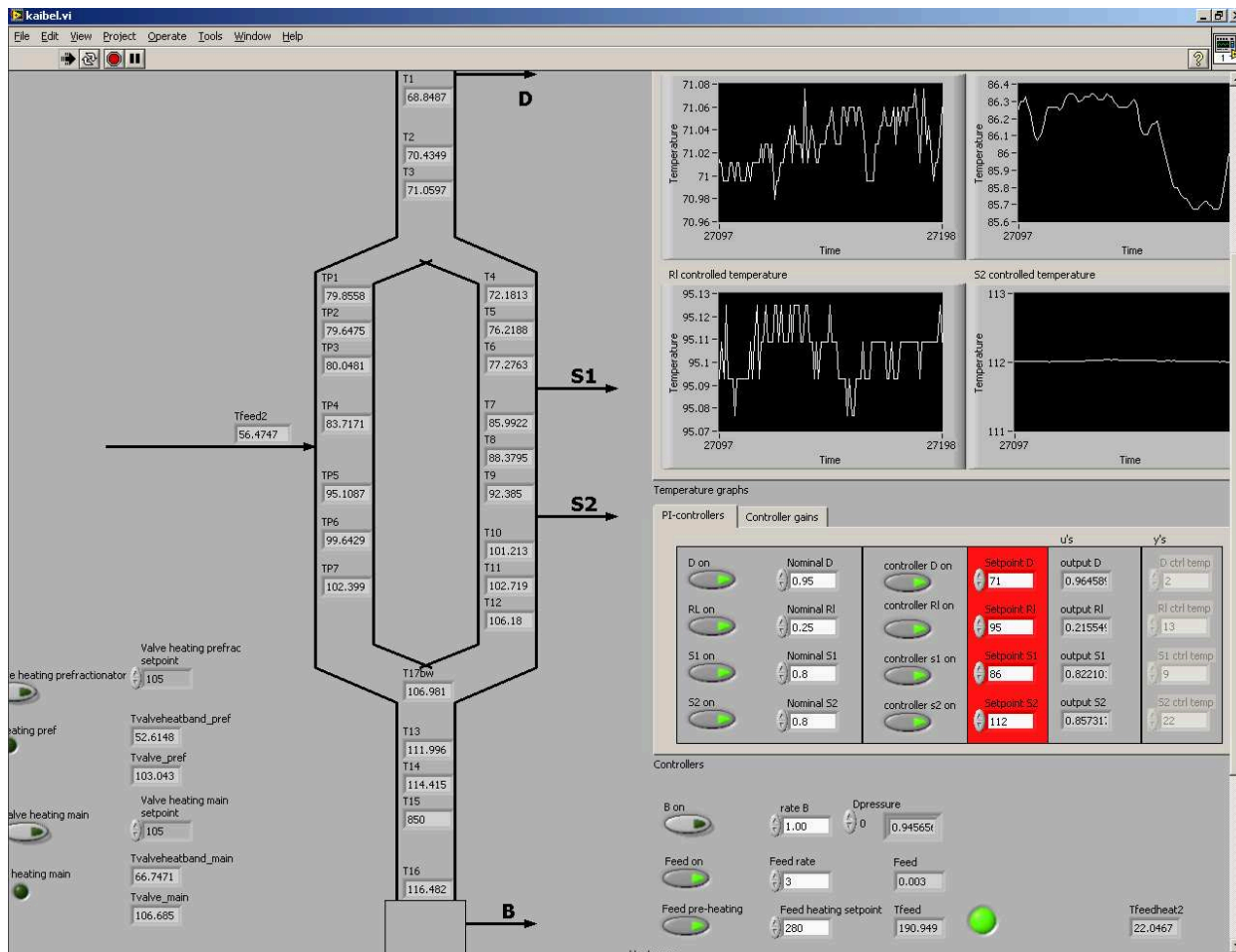
Figure 4: Screen-shot of operator interface during experimental run 12.
