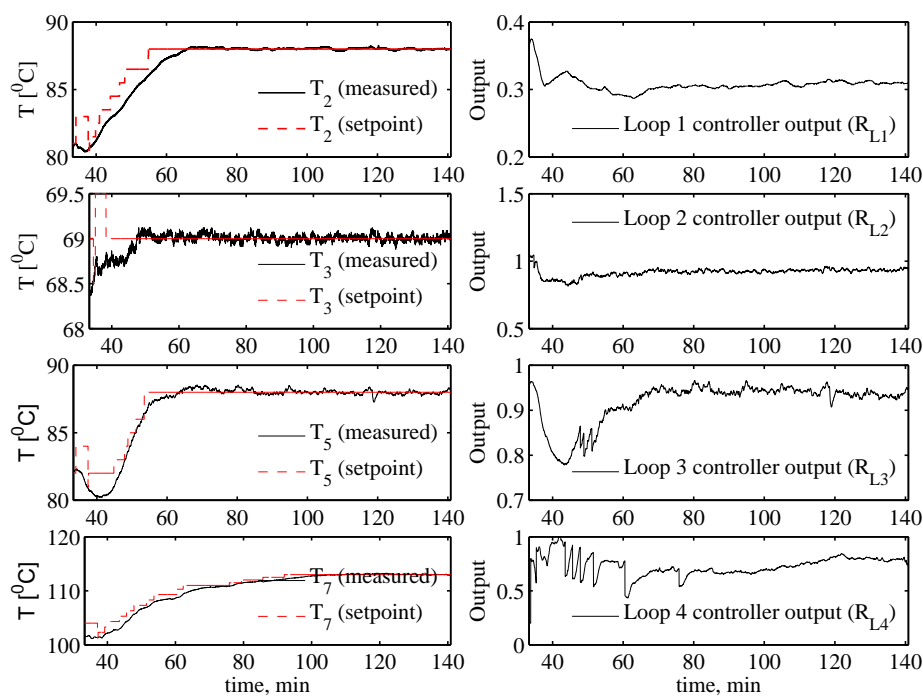
Figure 5: Experimental Run 1: Cold Start-up
