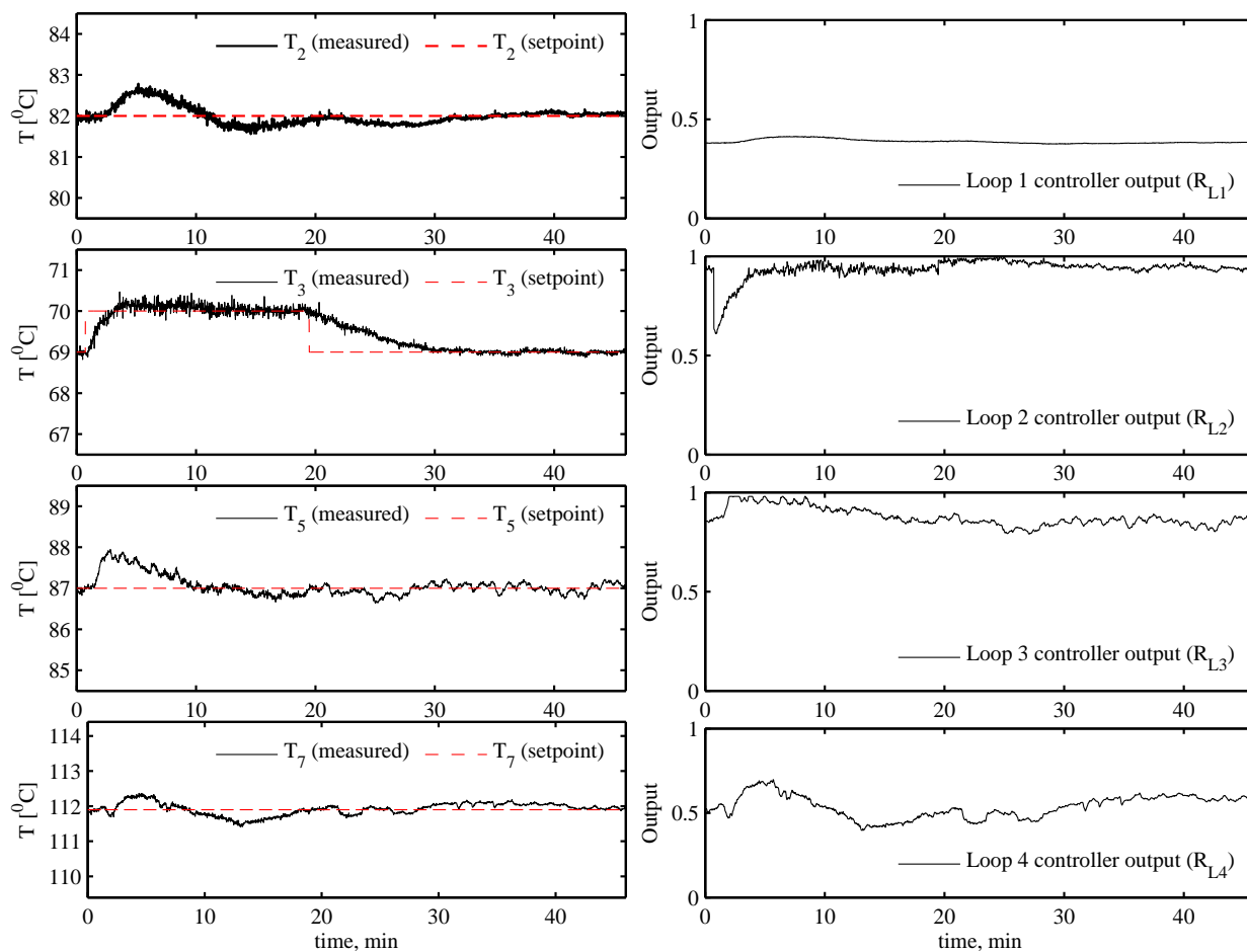
Figure 7: Experimental Run 3: \pm 1 ^{\circ}\text{C} setpoint change in top section temperature, T_3 (control loop 2)
