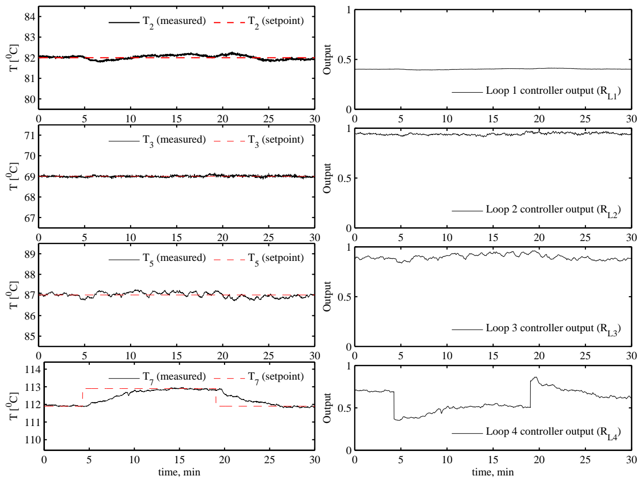
Figure 9: Experimental Run 5: \pm 1 ^{\circ}\text{C} setpoint change in bottom section temperature T_7 (control loop 4)
