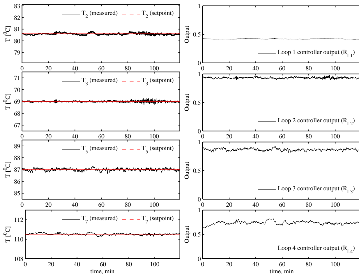
Figure 12: Experimental Run 8: steady state operation ( T_{2S} = 80.6^{\circ}\text{C} , T_{3S} = 69^{\circ}\text{C} , T_{5S} = 82^{\circ}\text{C} & T_{7S} = 110.2^{\circ}\text{C} )
