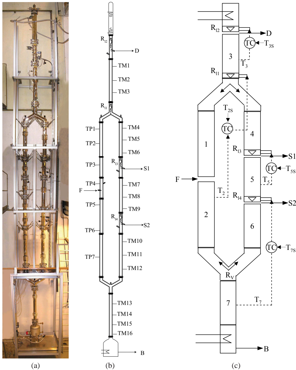
Figure 3: (a) Picture of the experimental column. 25 (b) Schematic showing location of temperature sensors. 25 (c) 4-point regulatory control structure used for operation T_2 = TP5 , T_3 = TM2 , T_5 = TM8 & T_7 = TM14 .
