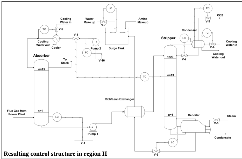
Resulting control structure in region I
