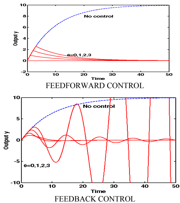
Figure 4. The problem with feedback... Comparison of feedforward and feedback control with respect to time delay error. Nominal delay \theta=0 .
