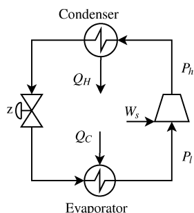
Figure 1. Simple refrigeration cycle with N_{ss}^{\max} = 5 potential degrees of freedom. However, if the flowsheet shows the actual process there will only be N_{ss} = 4 degrees of freedom, because there is no means of changing the active charge for example by filling or removing refrigerant.
