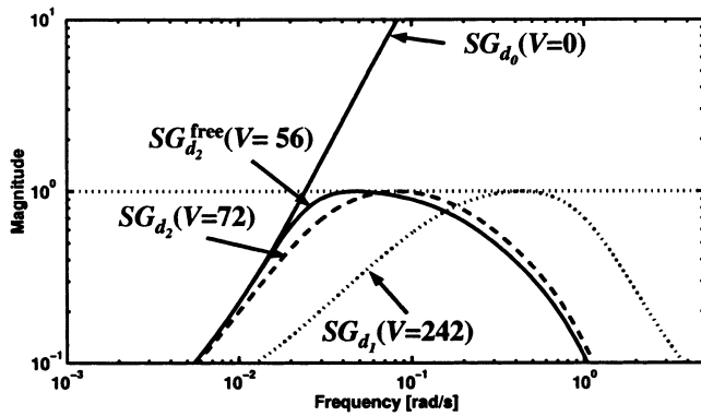
Figure 9. A buffer tank is needed for the temperature control problem: |SG_{d_0}| > 0 for frequencies above 0.024 rad/s. Comparison of |SG_{d_i}| = |SG_{d_0}h| for designs 1–3 in Table 2.
