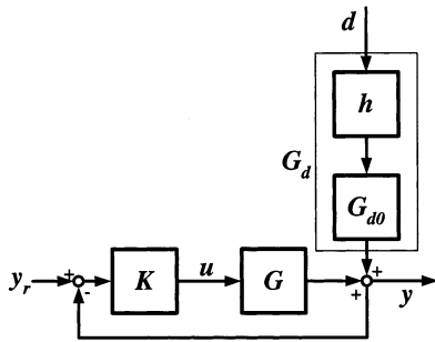
Figure 6. Feedback control system.
