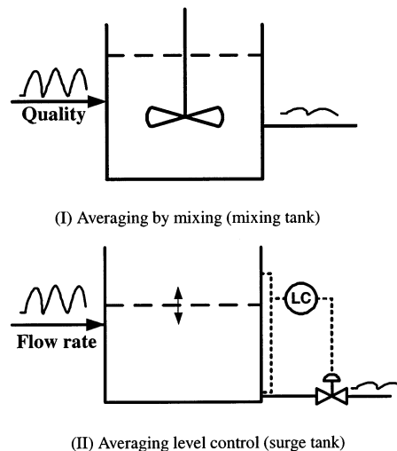
Figure 1. Two types of buffer tanks.
