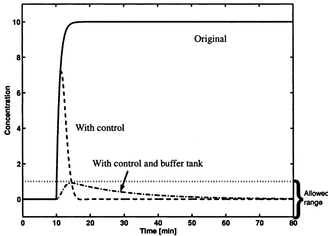
Figure 3. Response of the excess outlet concentration to a step in inlet quality (from 100 to 120 mol of A/m 3 at 10 min) for the system in Figure 2. A composition controller handles the long-term (“slow”) disturbance, but a buffer tank is required to handle the short-term deviations. Nominal data: q_A = 0.5 m 3 /min, q_B = 0.5 m 3 /min, c_A = 100 mol of A/m 3 , c_B = 100 mol of B/m 3 , c_0 = 0 mol of A – B/m 3 . Residence time mixer: 1 min. Delay in control loop \theta = 1 min. The levels in the mixer and the buffer tank are controlled by adjusting the outflow with PI controllers, k(s) = (50s + 1)/50s .
