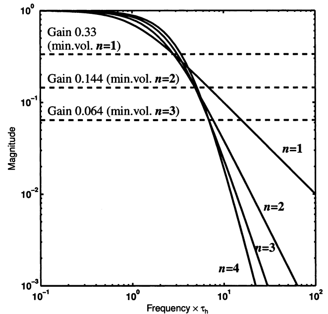
Figure 5. Frequency responses for h(s) = 1/[(\tau_h/n)s + 1]^n .
