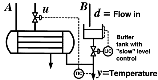
Figure 8. Temperature control with flow-rate disturbance.
