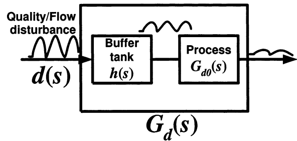
Figure 4. Use of buffer tank to dampen the disturbance.
