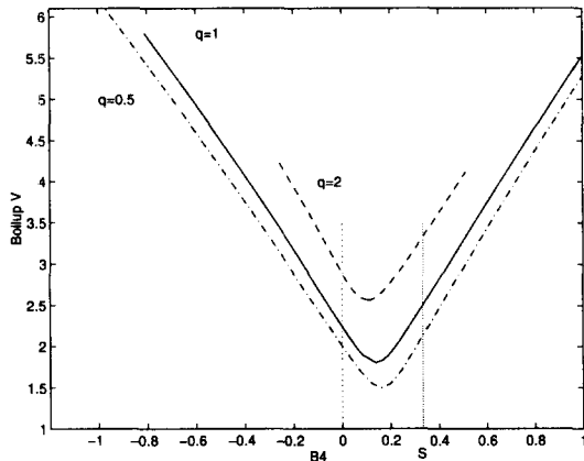
Fig. 9 Boilup as function of net downwards flow above the side stream ( B_4 ) in the “bad” PQ direction of the solution surface (recall Fig. 4).
