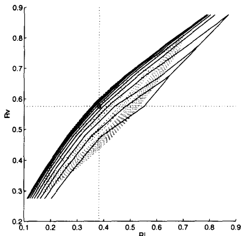
Fig. 12 Operating lines R_1=f(R_v) when DT_s=k for some values of k . Contour lines for constant V is shown dotted. (Feed is saturated liquid, q=1 )
