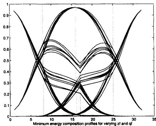
Fig. 10 Composition profiles for varying disturbances
