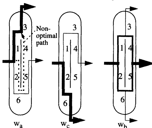
Fig. 8 Components taking "shortest" way through
