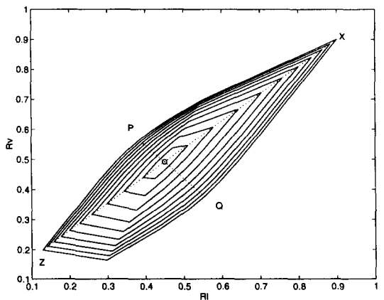
Fig. 5 Contour plot of V=J(R_I, R_V) . q=0.5 (Note that the change in boilup between contour lines is not constant, but quadratic)
