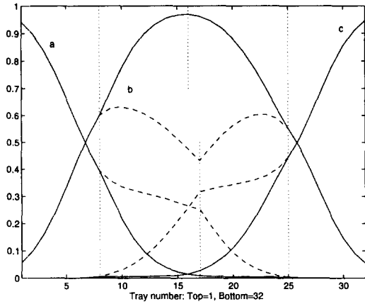
Fig. 2 Compositions of components a, b and c in prefractionator (dashed) and main column (solid).
