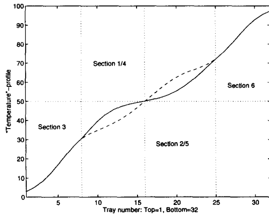
Fig. 3 Temperature profile in prefractionator (dashed) and main column (solid)
