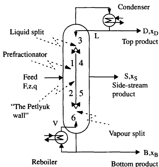
Fig. 1 The Petlyuk Distillation Column
