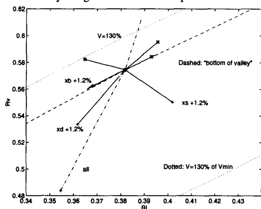
Fig. 6 Effect on optimal [R_l, R_v] from setpoint changes in product purity (96%-98.2%, 97% in the "centre").
