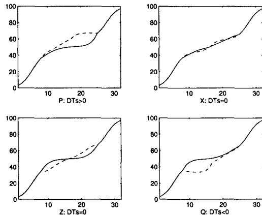
Fig. 11 Temperature profiles for off-optimal operation in directions along the bottom valley (ZX) and in the bad direction perpendicular to the valley (PQ).
