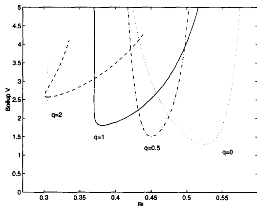
Fig. 7 Solution surface dependence of feed enthalpy factor. Projection into vertical plane through PQ.
