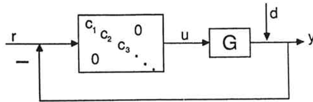
Figure 1. Decentralized control structure.
