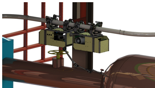
Fig. 1. Illustration of DORIS operation in a production plant.
