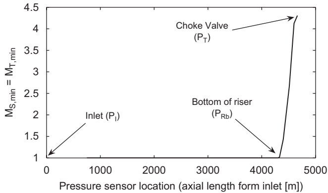
Fig. 10. Minimum peaks on |S| and |T| (as given by the relative distance between RHP-poles p and RHP-zeros z ) as function of pressure sensor location in pipeline.
