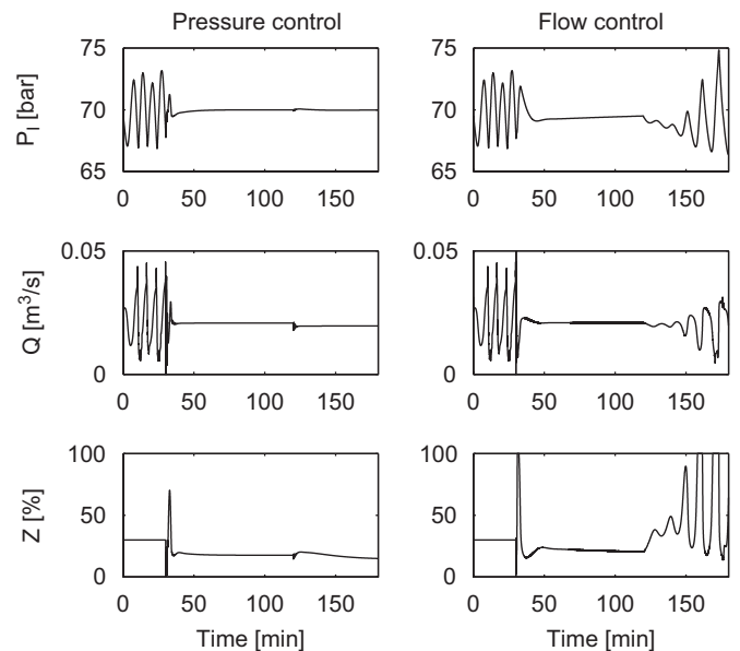
Fig. 16. Simulation of step in liquid feed at t = 120 min illustrating low-frequency disturbance rejection problems with flow control.
