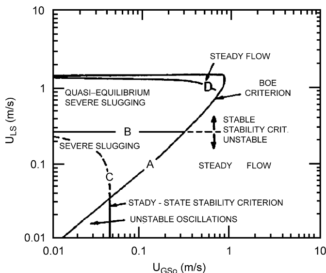
Fig. 1. Flow regime map for an experimental pipeline-riser system (Taitel, 1986). The map shows the flow regime in the pipeline as function of superficial gas and liquid velocities. Low gas and liquid velocities results in riser slugging.
