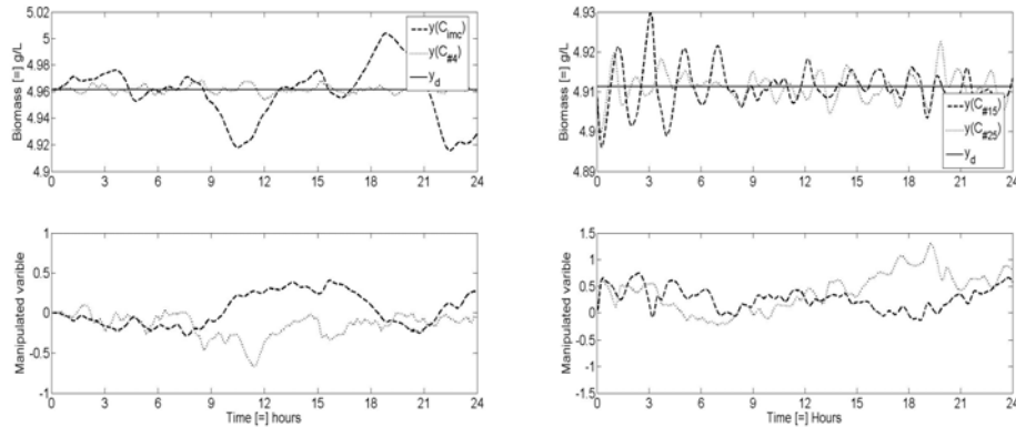
(a) Noisy simulation of the closed loop system at dilution rate 0.7 \text{ h}^{-1} with the initial IMC controller and the fourth iterate from the IFT tuning method. (b) Noisy simulation with an initial negative step disturbance to the closed loop system at dilution rate 0.795 \text{ h}^{-1} with the iterate no. 15 and 25 from the IFT tuning method.
