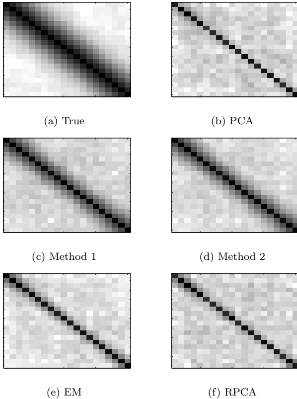
Fig. 1. Mean value over N_{mc} = 100 Monte Carlo simulations on the magnitude of each entry of \bar{\Psi} for each method
