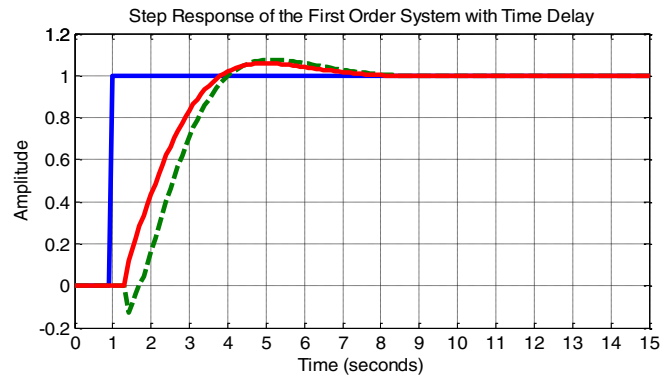
Fig. 8. Closed-loop response of the first order system.
