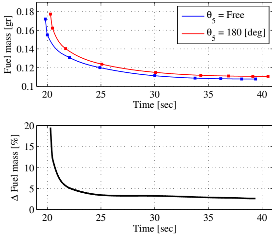
Fig. 3. Trade-off between fuel consumption and cycle time. Fuel consumption increases in all cycles when \theta_5 = 180 \text{ [deg]} .
