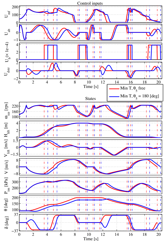
Fig. 4. min T controls and states for fixed and free \theta_5 . The dash-dotted lines are phase boundaries.
