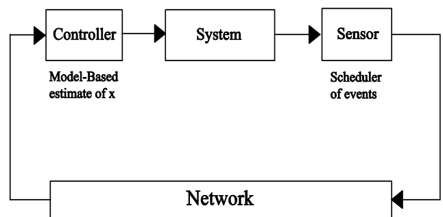
Fig. 1. Model-based event-triggered networked architecture
