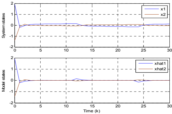
Fig. 2. Response of the real uncertain system with limited feedback (top). States of the model used to control the system (bottom)
