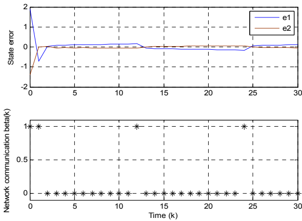
Fig. 3. State error used to determine the instants at which a feedback measurement has to be transmitted (top). Communication pattern \beta(k) (bottom)
