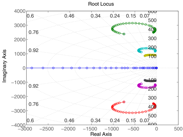
Fig. 5. Root Locus with a PFMP with the closed-loop characteristics equation
