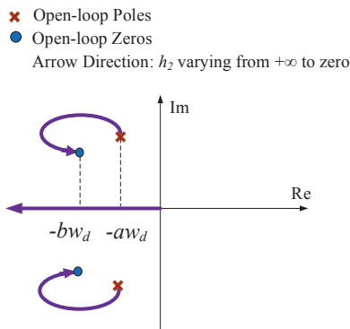
Fig. 4. Root Locus with a PFSP
