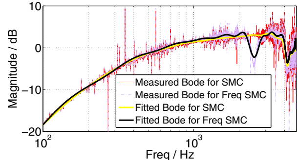
Fig. 9. Measured Frequency Response Plot from Vibration 3 to PES
