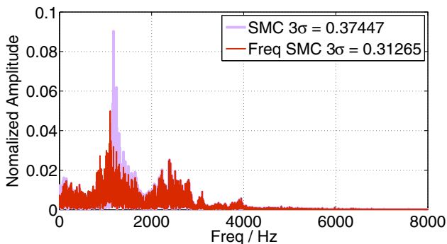
Fig. 6. PES Spectrum with Audio Vibration 1
