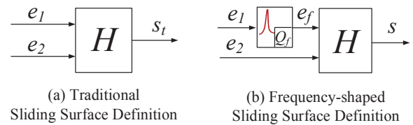
Fig. 2. Sliding Surface Definition
