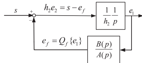
Fig. 3. Dynamics of Sliding Surface
