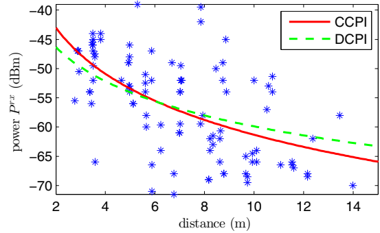
Fig. 4. Channel model identification with the CCPI (solid red line) and the DCPI (dashed green line) algorithm. The blue stars are the points of the RSS data set.
