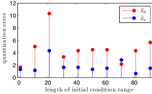
Fig. 3. Quantization error \tilde{x} = \mathbb{E}[\|\tilde{x} - N^{-1}\mathbf{1}\mathbf{x}(0)\|] for N = 7 nodes: deterministic ( \tilde{x}_d ) and a probabilistic ( \tilde{x}_u ) quantizer of uniform distribution for different values of the initial condition range L = 2x_0 , where \mathbf{x}(0) \sim U([-x_0, x_0]) , x_0 \in \{1/2, 11/2, \dots, 91/2\} .
