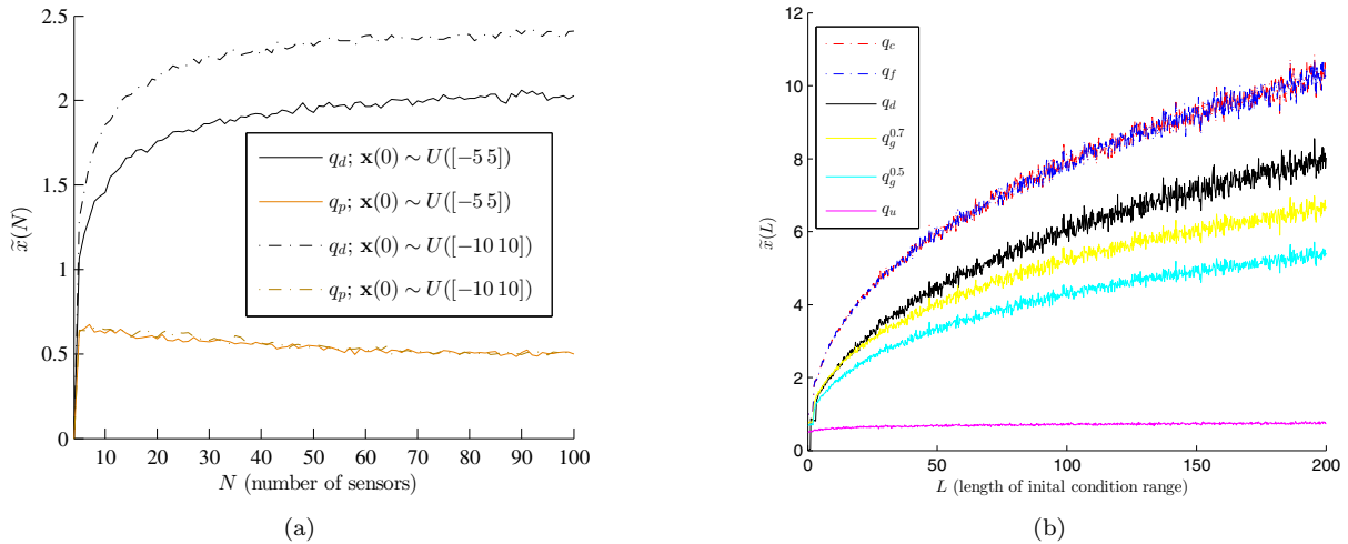
Fig. 1. Deterministic and probabilistic quantizers. (a) Comparison in terms of the deviation \tilde{x} between q_d and q_p , for complete graphs of N sensors. The plotted values are averaged over 1000 runs. The initial conditions are chosen from a uniform distribution on the given intervals. (b) Comparison in terms of \tilde{x} as a function of the length of initial condition range L = 2x_0 , where \mathbf{x}(0) \sim U([-x_0, x_0]) , x_0 \in [0, 100] , for different initial conditions and complete graphs ( N = 30 ). The plotted values are the average of 10000 runs.
