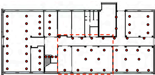
Fig. 2. Planimetry of the testbed (WSN layout).
