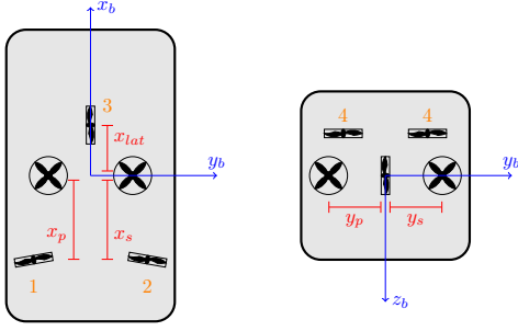
Fig. 2. Minerva schematic. Blue lines indicate coordinate axes in the b-frame. Red lines show thruster offsets.
