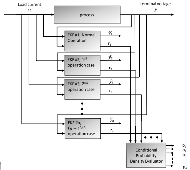
Fig. 3. Multiple-model residual generation and probability evaluation
