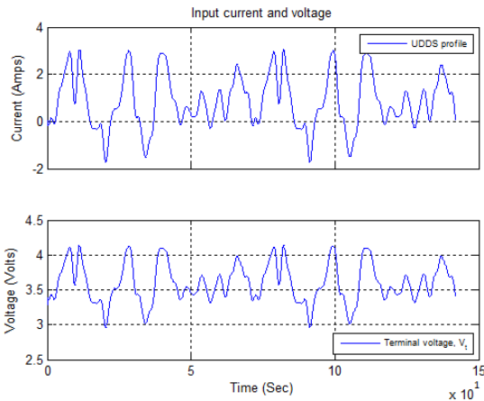
Fig. 6. UDDS load/charge current and terminal voltage profile
