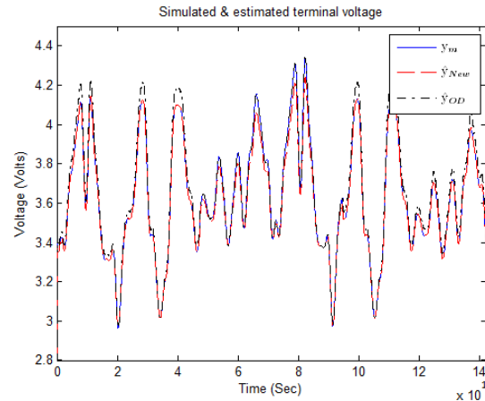
Fig. 7. Simulated and estimated terminal voltages
