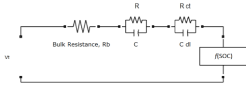
Fig. 1. Li-ion battery equivalent circuit model
