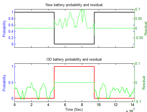
Fig. 8. Conditional probability density and residuals evaluated for new and OD battery condition
