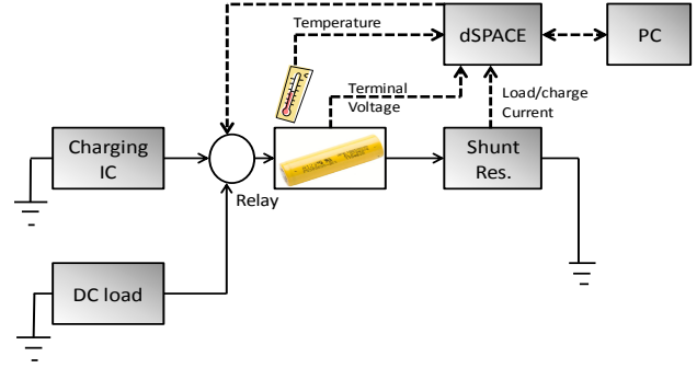
Fig. 4. Li-ion battery testing setup
