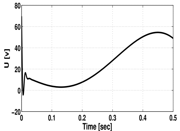
Fig. 7. Control voltage- Case with uncertain k , \eta , f_d
