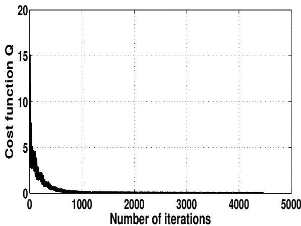
Fig. 4. Cost function
