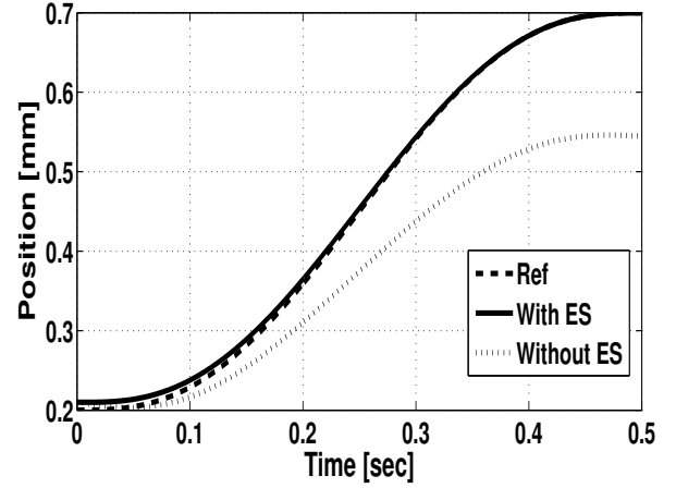
Fig. 1. Obtained Armature Position vs. Reference
