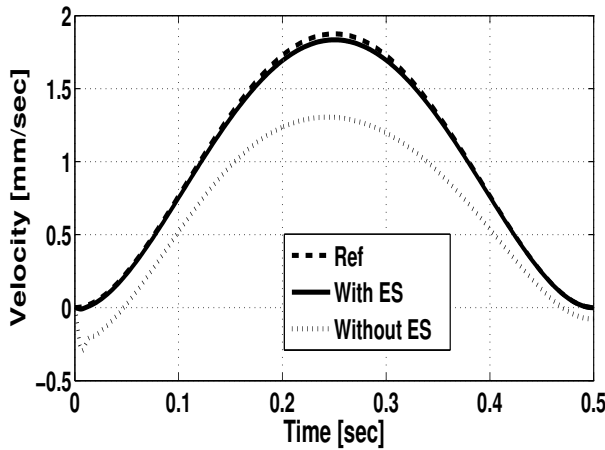
Fig. 2. Obtained Armature Velocity vs. Reference Trajectory
