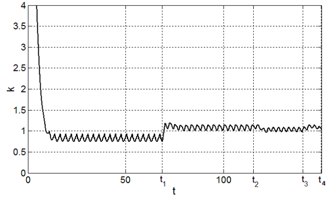
Fig. 2. Evolution of k(t) .
