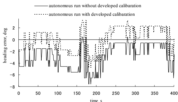
(b) Heading error in autonomous run
