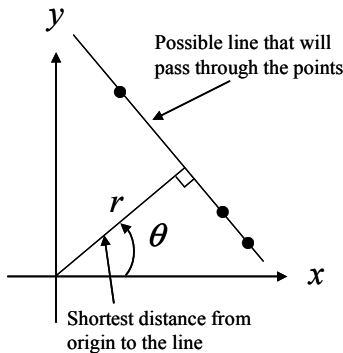
(a) r - \theta space normal representation of a line in Hough transform
