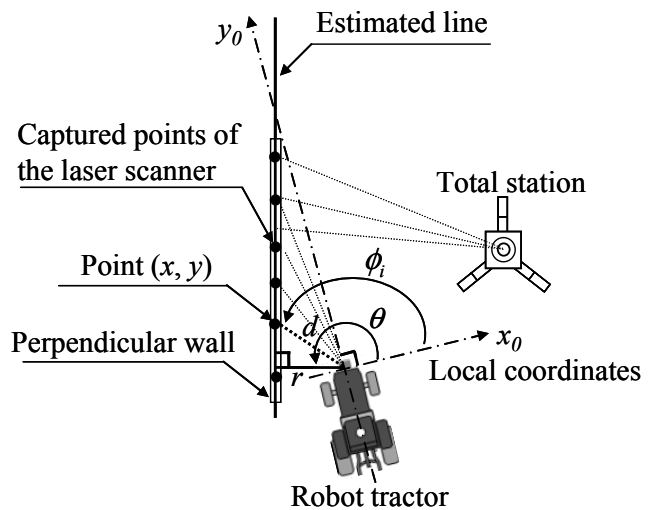
Fig. 3. Outline on how to recognize the perpendicular wall as straight line using the Hough transform
