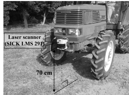
(b) Attachment position of laser scanner
