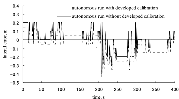
(a) Lateral error in autonomous run
