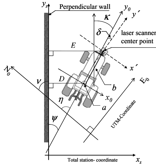
Fig. 5. Calibration method outline using a perpendicular wall as the reference line for getting the laser scanner exact position
