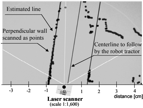
(a) Actual captured points by the laser scanner in a computer window
