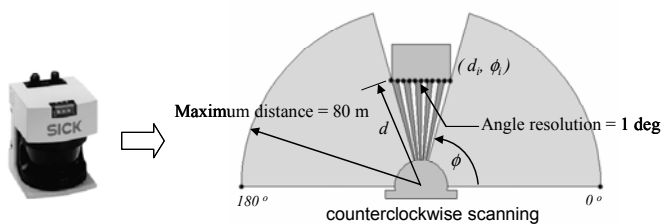
(a) Laser scanner (LMS 291) and scanning basic principles
