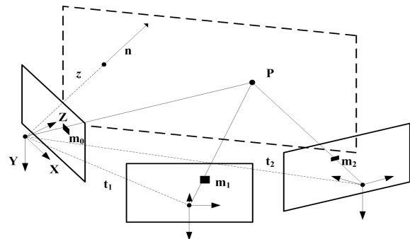
Fig. 4. Scheme of the geometry of multiple views of the same plane z.
