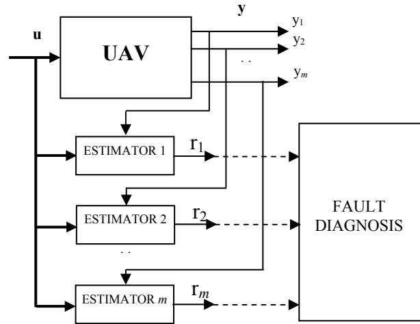
Fig. 1. Bank of estimators for output residual generation.
