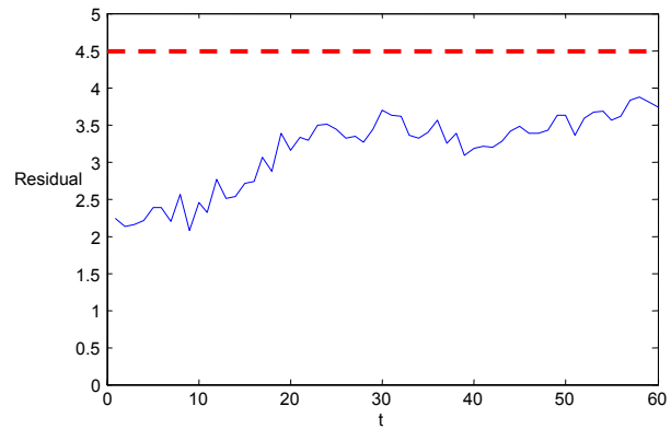
Fig. 7. Residuals for position estimation sequence with initial standard deviations of UDev=5.8 and VDev=6.1 , and threshold level of 4.5.
