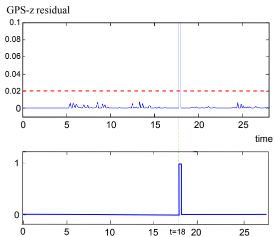
Fig. 2. Outlier GPS-z sensor failure detection. Upper plot: residual signal. Lower plot: fault detection signal.
