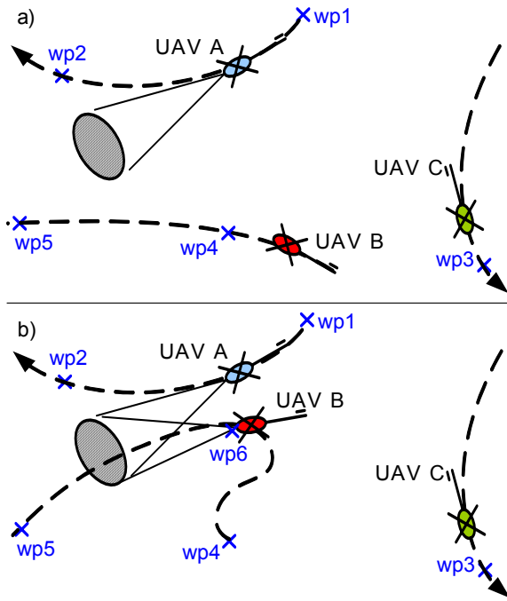
Fig. 6. An example illustrating the re-planning process: a) UAVs following the initial plan. b) Dynamic replanning: UAV B plan changes to go to wp6.
