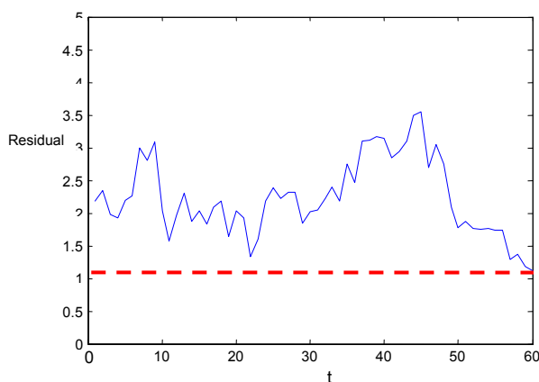
Fig. 8. Residuals for position estimation sequence with initial standard deviations of UDev=2.3 and VDev=1.5 , and threshold level of 1.5.
