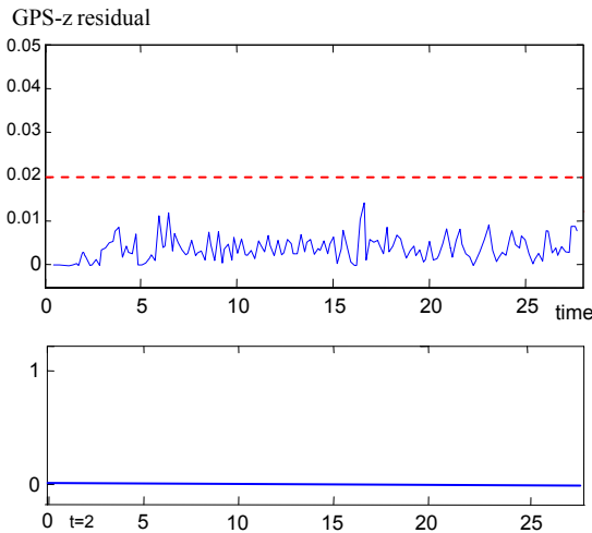
Fig. 3. Slow-growing drift GPS-z sensor failure detection. Upper plot: residual signal. Lower plot: fault detection signal.
