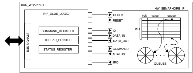
Fig. 6. Overview of the hardware semaphore organization.
