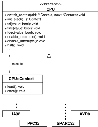
Fig. 2. Overview of the CPU hardware mediator.
