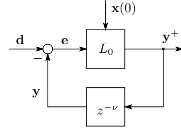
Fig. 2. Equivalent system with the biproper system L_0 .
