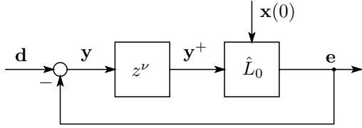
Fig. 3. Equivalent system with the inverse system \hat{L}_0 of L_0 .
