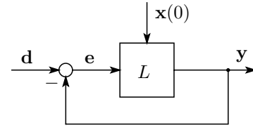
Fig. 1. Discrete-time feedback control system.
