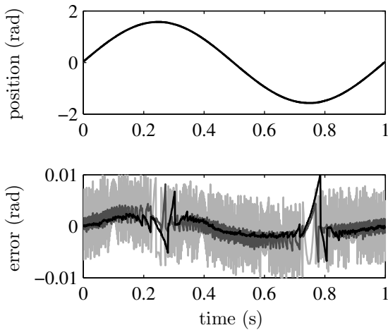
Fig. 6. Position signals, reference (dashed), quantized measurement (light grey), estimated with \sigma = 0 counts (dark grey) and with \sigma = 3 counts (black).
