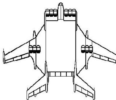
Fig. 2. Ekranoplane with "combined wing" configuration
