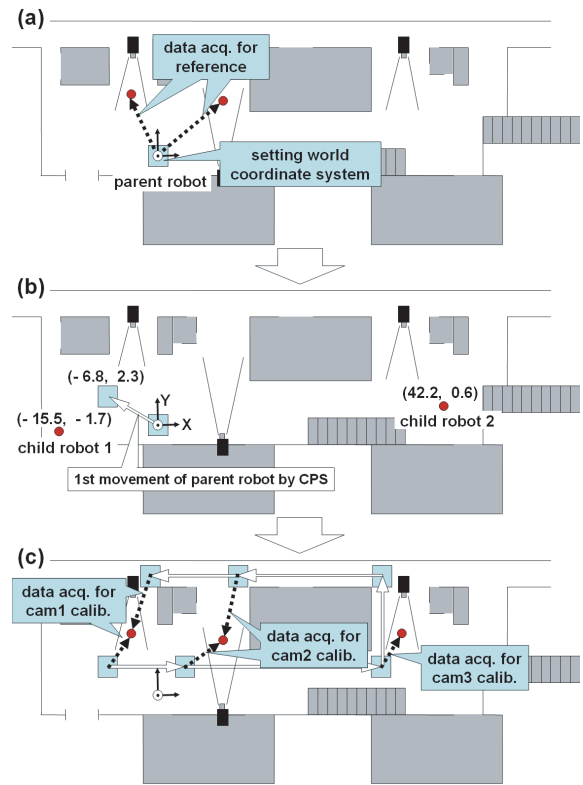
Fig. 11. Experiment sequence of cooperative positioning and data acquisition for camera calibration
