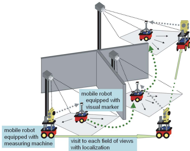
Fig. 1. Calibration of distributed vision network by a group of mobile robots
