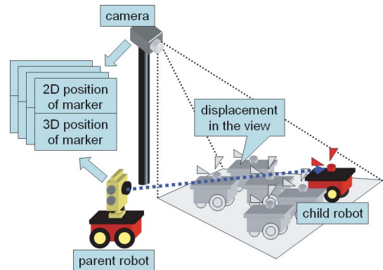
Fig. 2. Data acquisition for camera calibration: position of visibly distinguishable marker on a child robot is measured by the camera while 3D position of the marker is measured by a parent robot using precision measuring machine.
