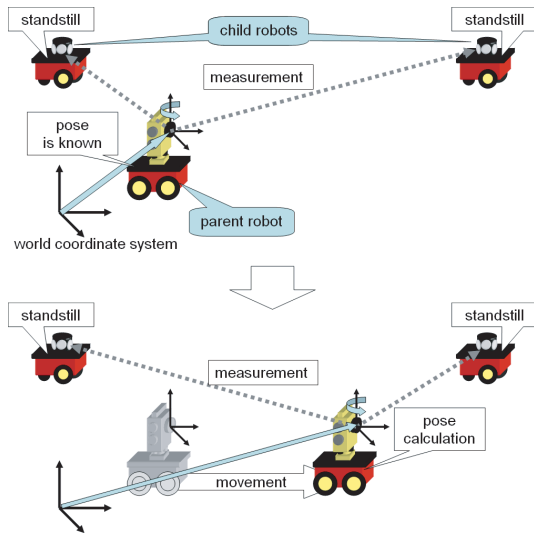
Fig. 4. Principle of cooperative positioning
