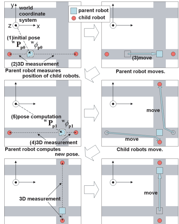
Fig. 5. Alternative move of parent robot and child robots in cooperative positioning in a passage of a building
