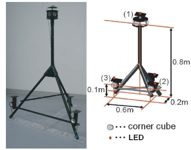
Fig. 6. Arrangement of LEDs and corner cubes
