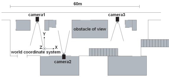
Fig. 9. Experiment setup (top view)
