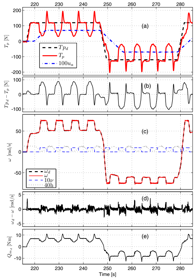
Fig. 5. Test with large thrust losses and without anti-spin: propeller thrust and advance speed (a), thrust error (b), shaft speed (c), shaft speed error (d) and desired motor torque (e).
