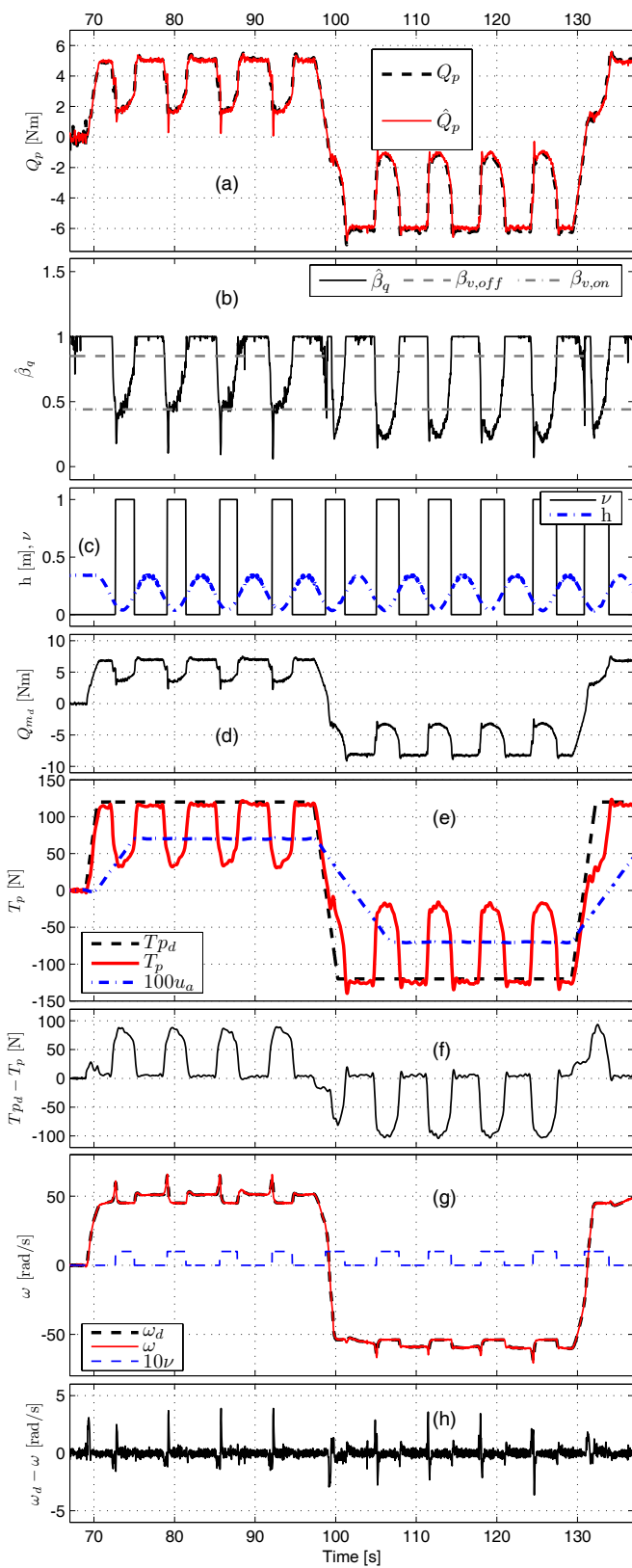
Fig. 4. Test with large thrust losses and anti-spin: propeller torque and its estimate (a), ventilation detection (b) and (c), desired motor torque (d), propeller thrust and advance speed (e), thrust error (f), shaft speed (g) and shaft speed error (h).
