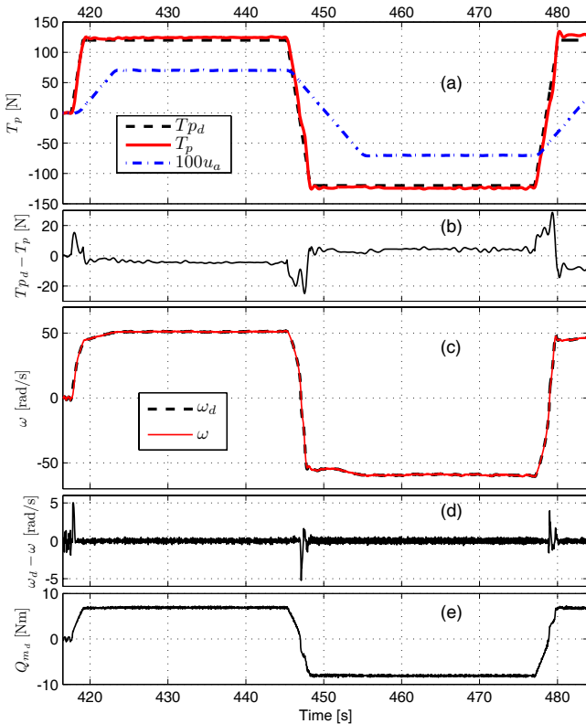
Fig. 3. Undisturbed water test: propeller thrust and advance speed (a), thrust error (b), shaft speed (c), shaft speed error (d) and desired motor torque (e).
