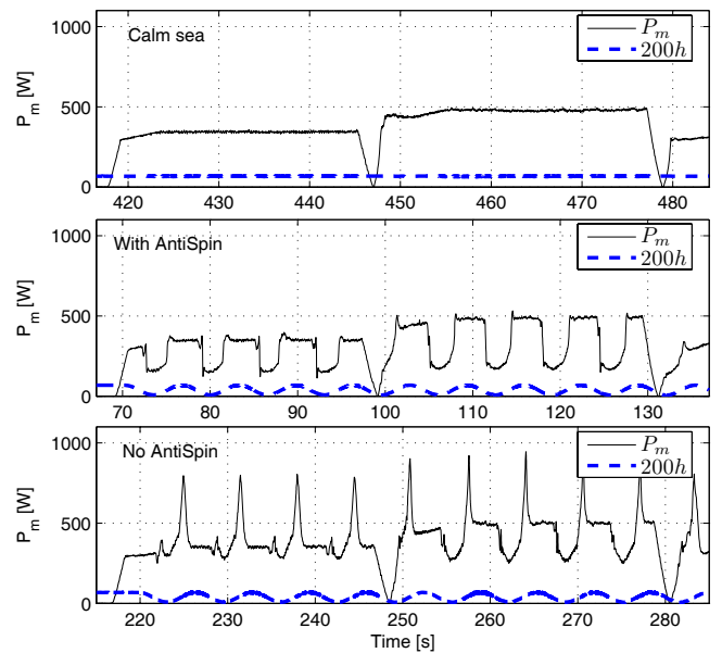
Fig. 6. Motor power in calm water and with large thrust losses (with and without the anti-spin algorithm).
