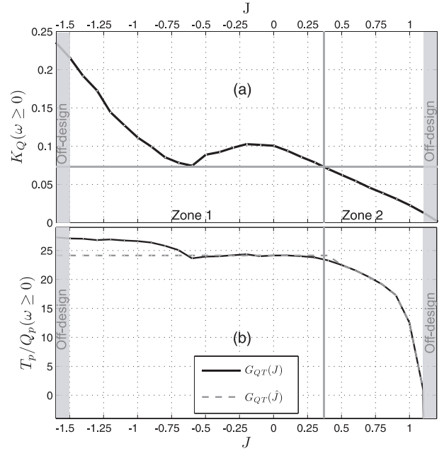
Fig. 2. K_Q characteristic for \omega \geq 0 and the ratio between thrust and torque for \omega \geq 0 .
