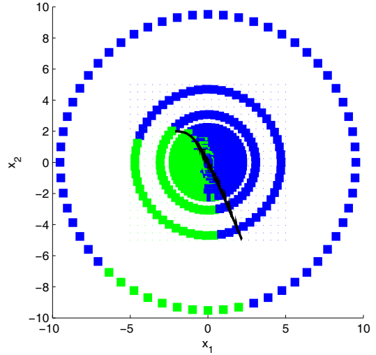
Fig. 6. Juxtaposition of the result in Corona et al. (2007) with the switching law obtained with the approximated criterion (6). The right and dark zone corresponds to \rho = 1 , and the left and light zone to \rho = 0 .
