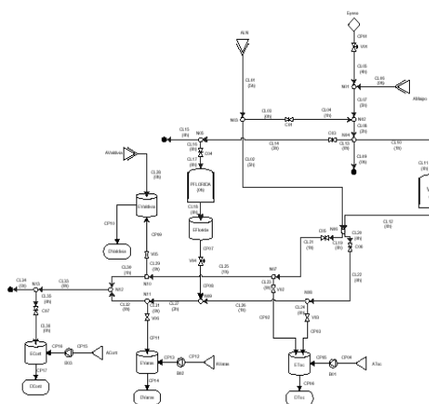
Fig. 2. Simplified version of the Santiago network
