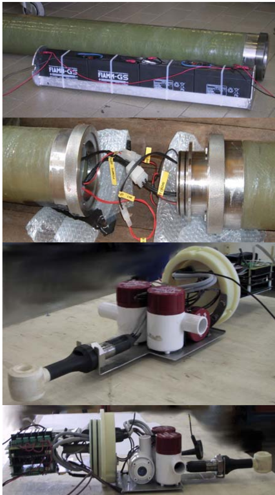
Fig. 2. Some realization details of the Følaga, second version. From top to bottom: mid section with battery pack lodging; central section, with mechanical, electrical and electronic connections; bow end-cap, wet side, with CTD sensor (the "nose"), and the two steering lateral jet pumps; again bow end-cap, side view, with the CTD, the lateral steering pumps and the vertical diving pump visible on the wet side (right), and the electronic package on the dry side (left). The connections through the cap between wet and dry sides have been coiled with epoxy.
