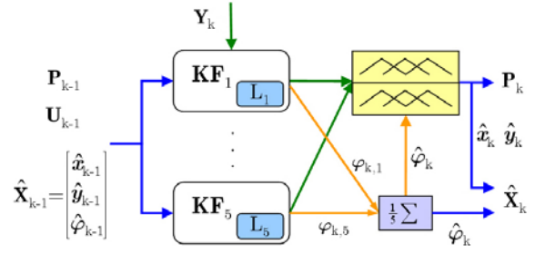
Fig. 7. Takagi-Sugeno based fuzzy observer.
