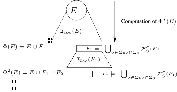
Fig. 2. \Phi^* Intuition from the point of view of G
