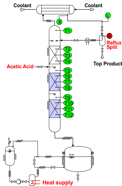
Fig. 2. Reactive Distillation Column
