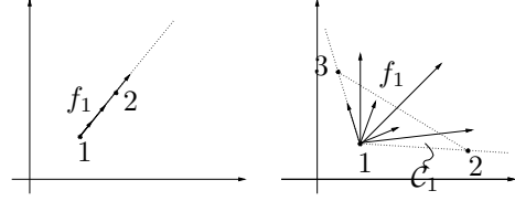
Fig. 2. Vector fields satisfying A2.
