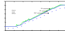
Fig. 9 Fuel feedback control by the PID controller ( P=2.3 , I=0.2 , D=0 )
