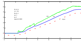
Fig. 18. Fuel loop feedback control by the NN-Tuning 2-DOF PID controller ( P=2.2 , I=1.1 , D=0.1 , w=1 , b=1 , epoch=500).
