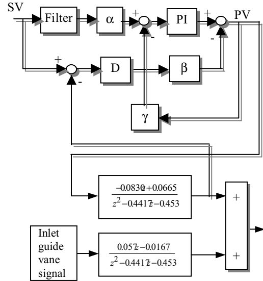
Fig. 3. The structure of 2-DOF PID controller for Gun-san gas turbine.
