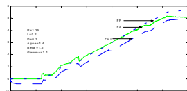
Fig. 14. Fuel loop feedback control by the conventional 2-DOF PID controller ( P=1.35 , I=0.2 , D=0.1 , \alpha=1.4 , \beta=1.2 , \gamma=1.1 ).
