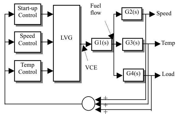
Fig. 2. Control system of the Gun-san gas turbine generating plant: VCE=fuel flow signal, G1(s)= transfer function of fuel system, G2(s)=transfer function between fuel flow and turbine speed, G3(s)=transfer function between fuel flow and turbine exhaust gas temperature, G4(s)=transfer function between fuel flow and generator output.
