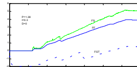
Fig. 11. Fuel loop feedback control by the PID controller in gas temperature ( P=1.38 , I=0.3 , D=0 ).
