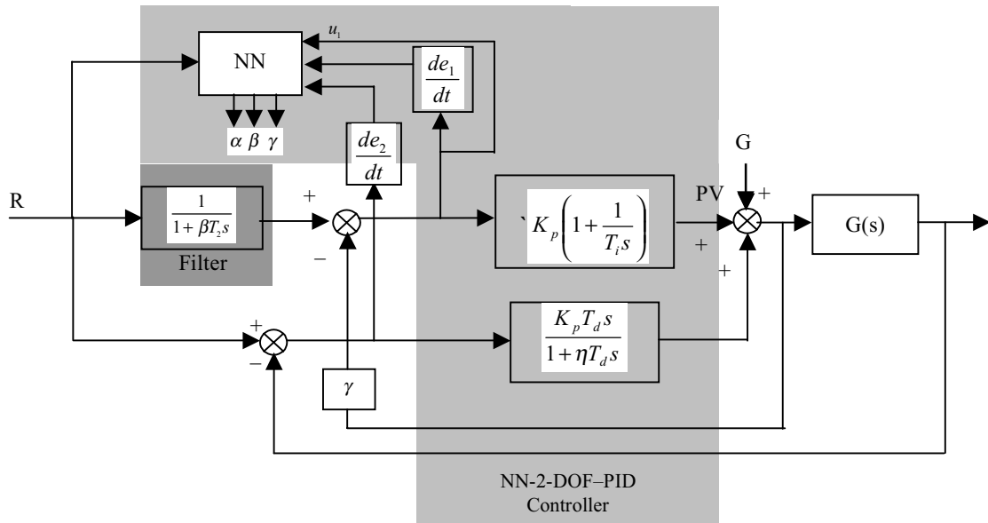
Fig.4 (a). The structure of the 2-DOF PID controller with a neural network for the Gun-san gas turbine.
