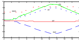
Fig. 7 Each parameter curve during the start-up, running and stop procedures of the Gun-san gas turbine.
