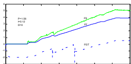
Fig. 12. Fuel loop feedback control by the PID controller in the event of a gas temperature disturbance ( P=1.56 , I=0.12 , D=0.0 ).
