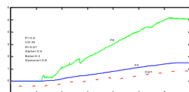
Fig. 16. Fuel loop feedback control by the conventional 2-DOF PID controller ( P=3.5 , I=0.32 , D=0.01 , \alpha=0.5 , \beta=0.3 , \gamma=0.8 ).
