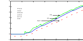
Fig. 21. Fuel loop feedback control by the NN-Tuning 2-DOF PID controller ( P=2.2 , I=0.2 , D=0.01 , w=0.2 , b=1.5 , h=5 ).
