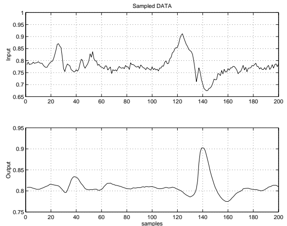
Fig. 2. Sampled data
