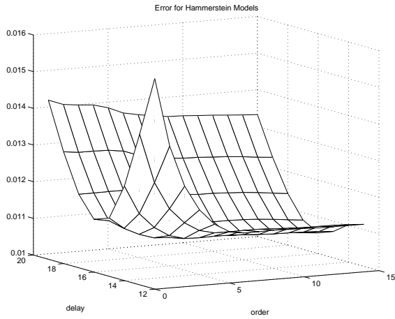
Fig. 4. Hammerstein Models
