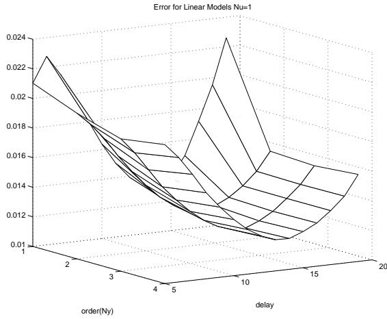
Fig. 3. Linear Models
