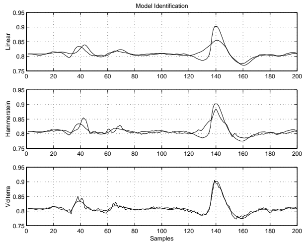
Fig. 7. Model Identification
