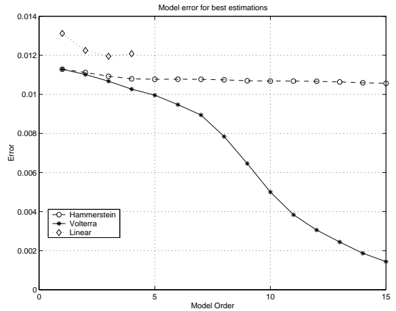
Fig. 6. Error comparison
