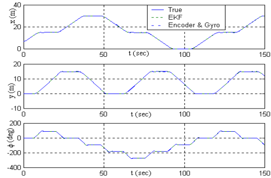
Fig. 6. The state changes of X, Y, and \Phi .
