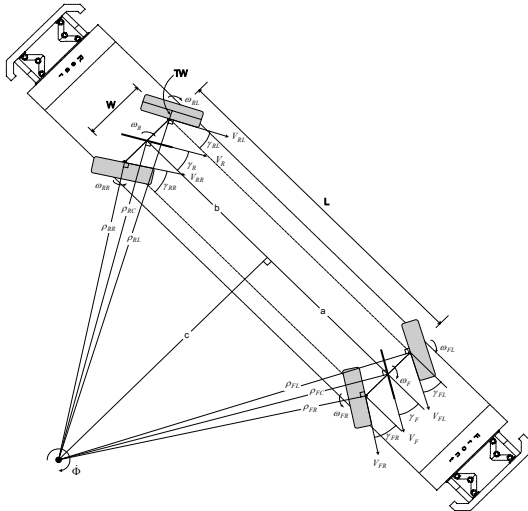
Fig. 2. Four-wheel steering AGV kinematic model.
