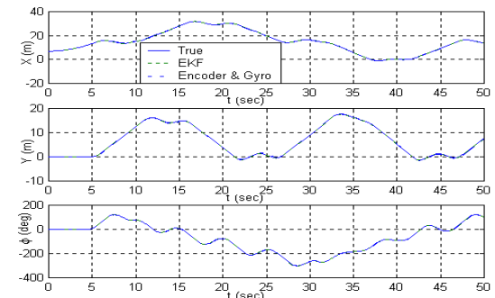
Fig. 10. The state changes of X, Y, \Phi .
