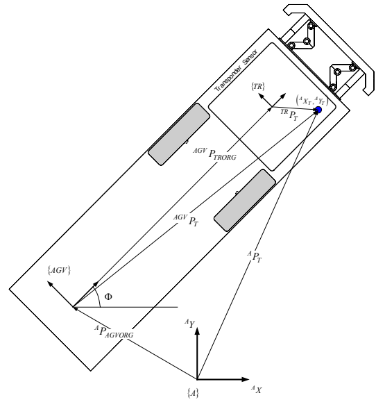
Fig. 4. Mounting of transponder sensor.
