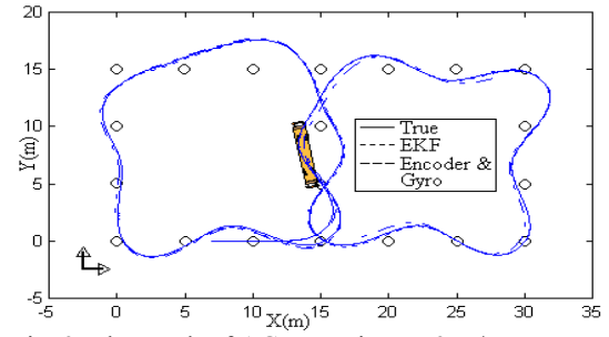
Fig. 9. The result of AGV running at 3 m/s.
