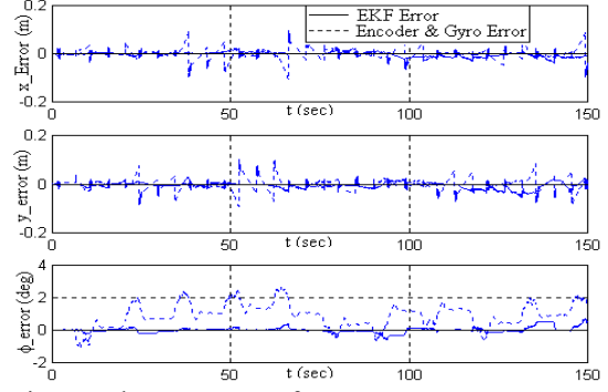
Fig. 7. The state errors of X, Y, \Phi .
