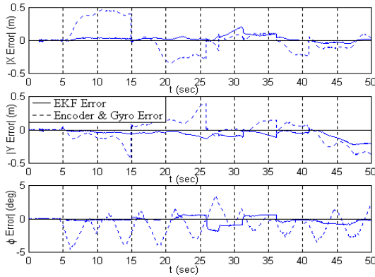
Fig. 11. The state errors of X, Y, \Phi .
