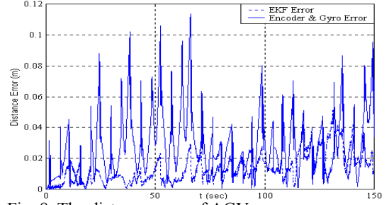
Fig. 8. The distance error of AGV.
