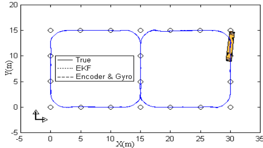
Fig. 5. The result of AGV running at 1m/s.
