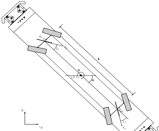
Fig. 3. Two wheel steering AGV Kinetic model.
