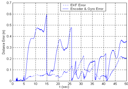
Fig. 12 The distance error of AGV.
