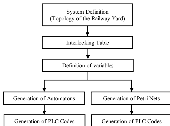
Fig. 10. Development steps for interlocking software.
