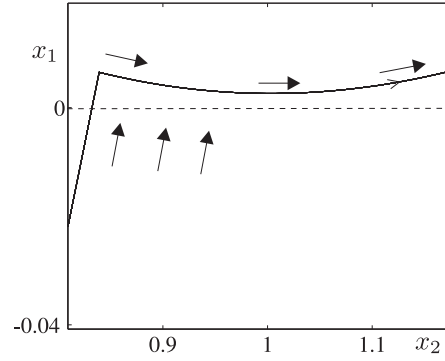
Fig. 4. Zoom into the neighbourhood of the switching surface of the periodic orbit from Figure 3 with digital sampling \tau = 0.005 .
