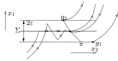
Fig. 7. Schematic representation of the bounding region along the limit cycle for sufficiently small sampling time \tau .
