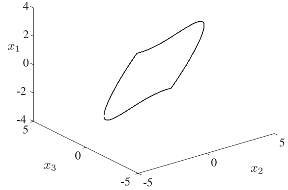
Fig. 1. Periodic orbit of system (10) with a segment of sliding when no digital sampling is applied to the system. Parameters are set to \zeta = 0.1 , \omega = 1 , k = 1 , \sigma = -1 and \rho = 0.4 .
