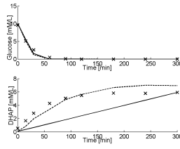
Figure 7. c_{GLC} and c_{DHAP} vs. time, exp. data: x, pure simulation: continuous line, one step ahead pred.: dashed
