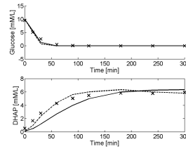
Figure 8. c_{GLC} and c_{DHAP} vs. time after modeling r_1 and r_2 , exp. data: x, pure simulation: continuous line, one step ahead pred.: dashed
