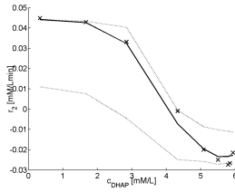
Figure 6. r_2 vs. c_{DHAP} , exp. data: x, local fit: continuous line and 95% conf. intervals: dashed
