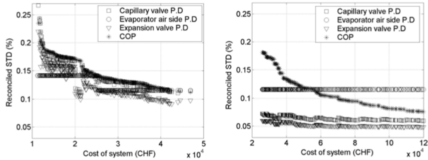
Figure 3. (left: Eq. 5, right: Eqs. 4 and 6) Trade-off curves for four KPI (100,000 evaluations)
