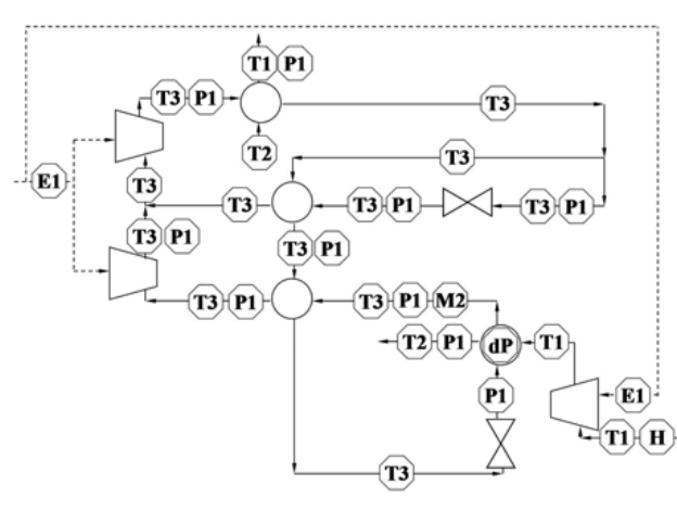
Figure 1. Air-water two stage heat pump
