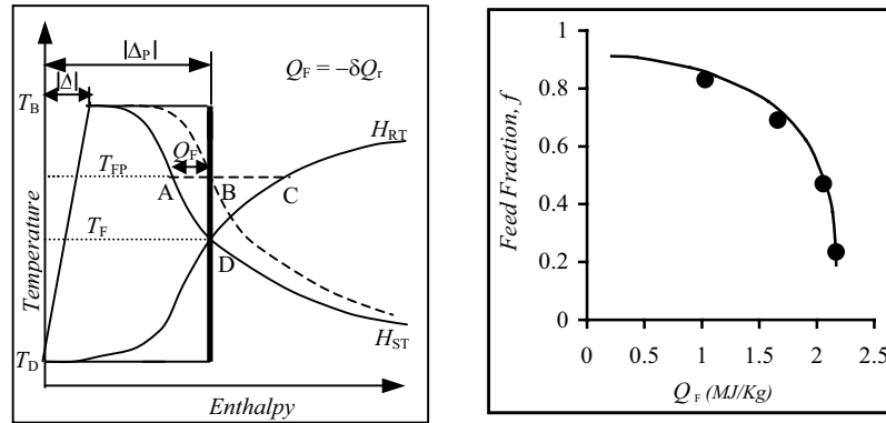
Figure 2. (a) Feed preheat targeting by feed splitting through composite IRS curves (b) Relation between feed split-fraction and preheat duty for the benzene-propane example
